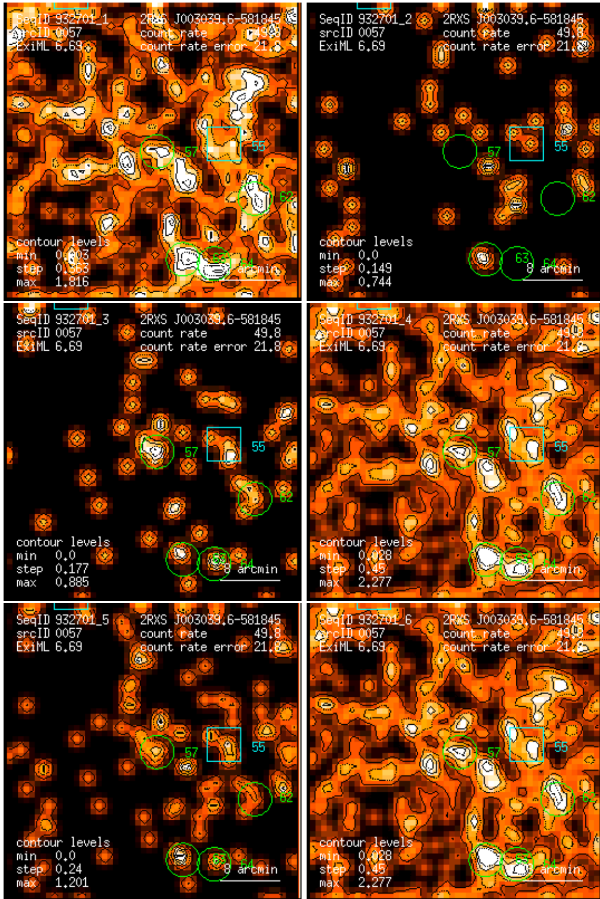
Figure 57: RASS 932701: detection 0057: band rate images, Gaussian filter: (1) PSPC channels 11 – 41, (2) 52 – 90, (3) 91 – 201, (4) 11 – 235, (5) 52 – 201, (6) 11 – 201. Broad band rates in counts/ks. Band rate contour levels in counts/ks/arcmin 2 .
