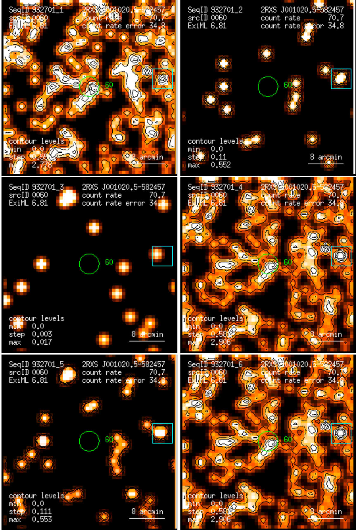
Figure 60: RASS 932701: detection 0060: band rate images, Gaussian filter: (1) PSPC channels 11 – 41, (2) 52 – 90, (3) 91 – 201, (4) 11 – 235, (5) 52 – 201, (6) 11 – 201. Broad band rates in counts/ks. Band rate contour levels in counts/ks/arcmin 2 .
