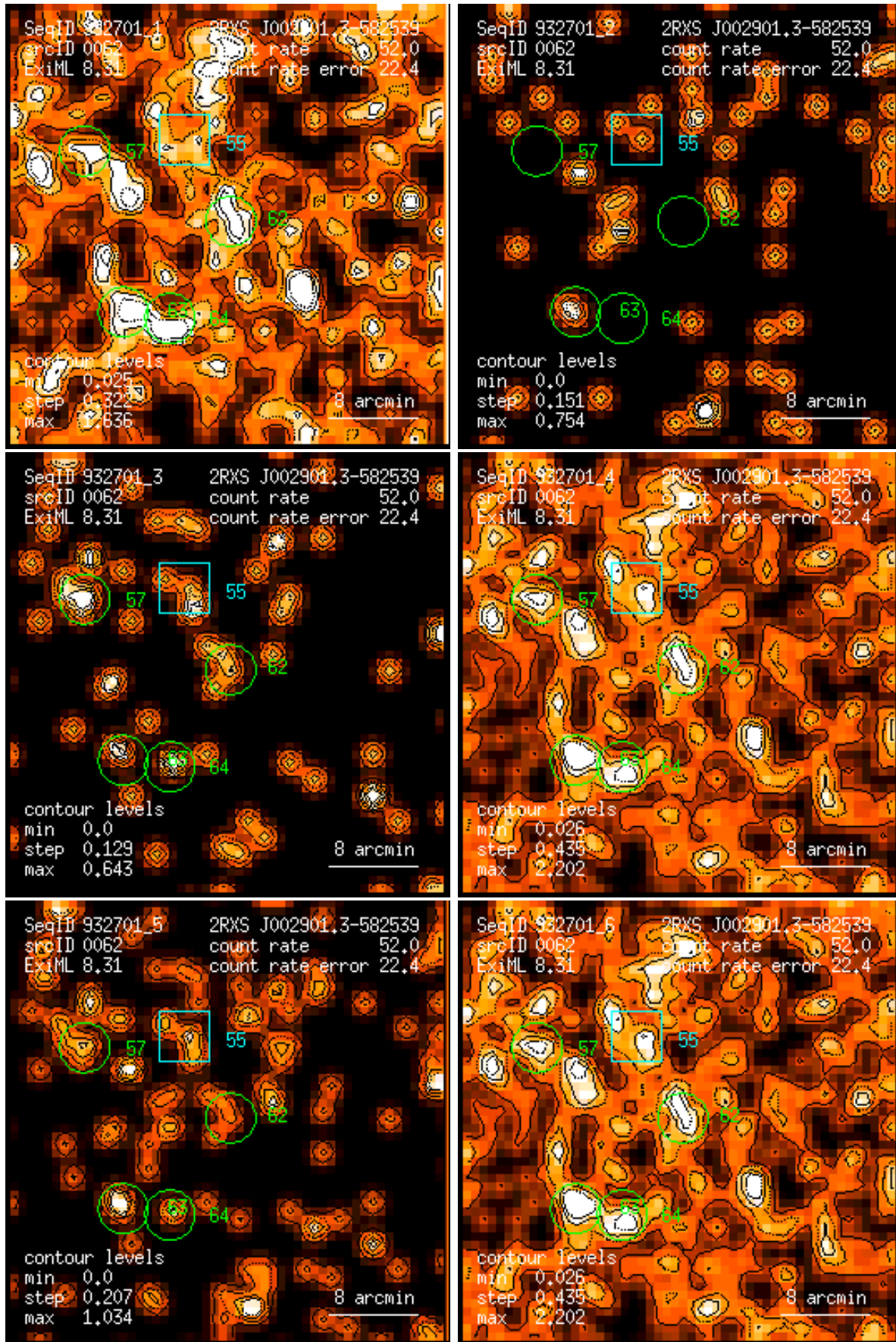
Figure 62: RASS 932701: detection 0062: band rate images, Gaussian filter: (1) PSPC channels 11 – 41, (2) 52 – 90, (3) 91 – 201, (4) 11 – 235, (5) 52 – 201, (6) 11 – 201. Broad band rates in counts/ks. Band rate contour levels in counts/ks/arcmin 2 .
