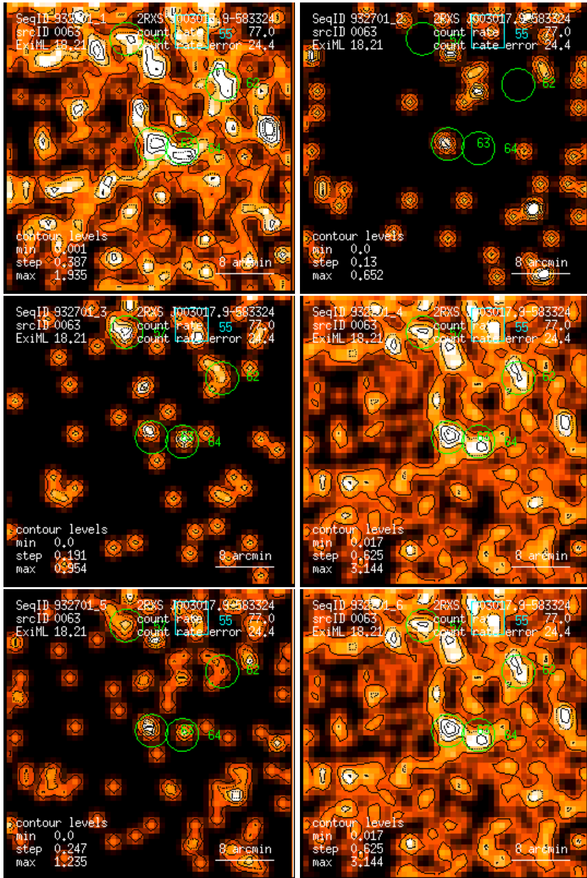
Figure 63: RASS 932701: detection 0063: band rate images, Gaussian filter: (1) PSPC channels 11 – 41, (2) 52 – 90, (3) 91 – 201, (4) 11 – 235, (5) 52 – 201, (6) 11 – 201. Broad band rates in counts/ks. Band rate contour levels in counts/ks/arcmin 2 .
