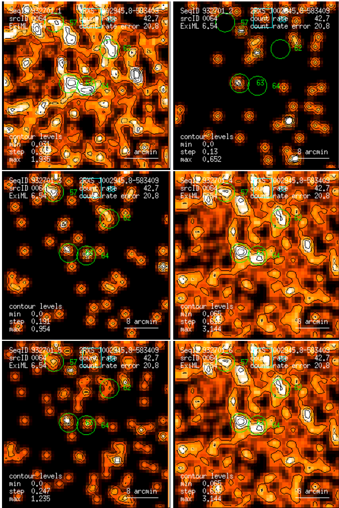
Figure 64: RASS 932701: detection 0064: band rate images, Gaussian filter: (1) PSPC channels 11 – 41, (2) 52 – 90, (3) 91 – 201, (4) 11 – 235, (5) 52 – 201, (6) 11 – 201. Broad band rates in counts/ks. Band rate contour levels in counts/ks/arcmin 2 .
