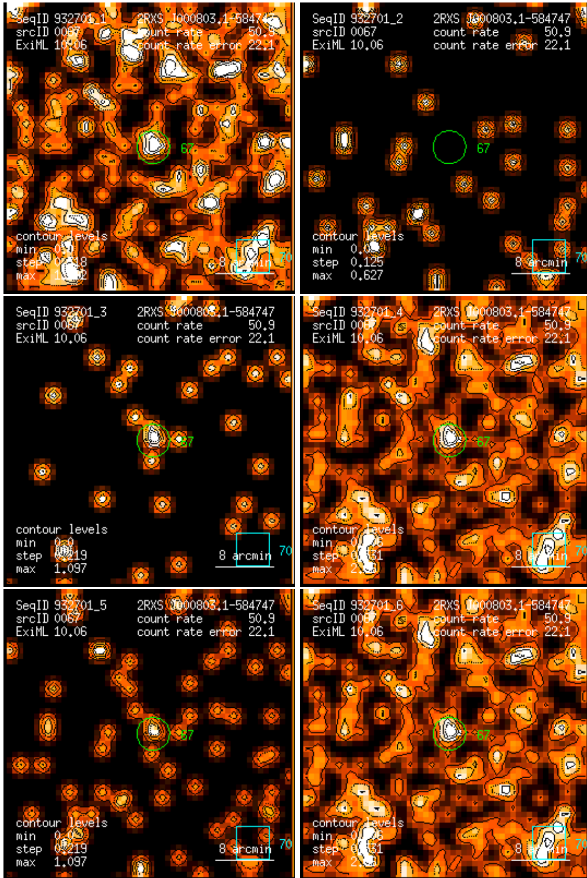
Figure 67: RASS 932701: detection 0067: band rate images, Gaussian filter: (1) PSPC channels 11 – 41, (2) 52 – 90, (3) 91 – 201, (4) 11 – 235, (5) 52 – 201, (6) 11 – 201. Broad band rates in counts/ks. Band rate contour levels in counts/ks/arcmin 2 .
