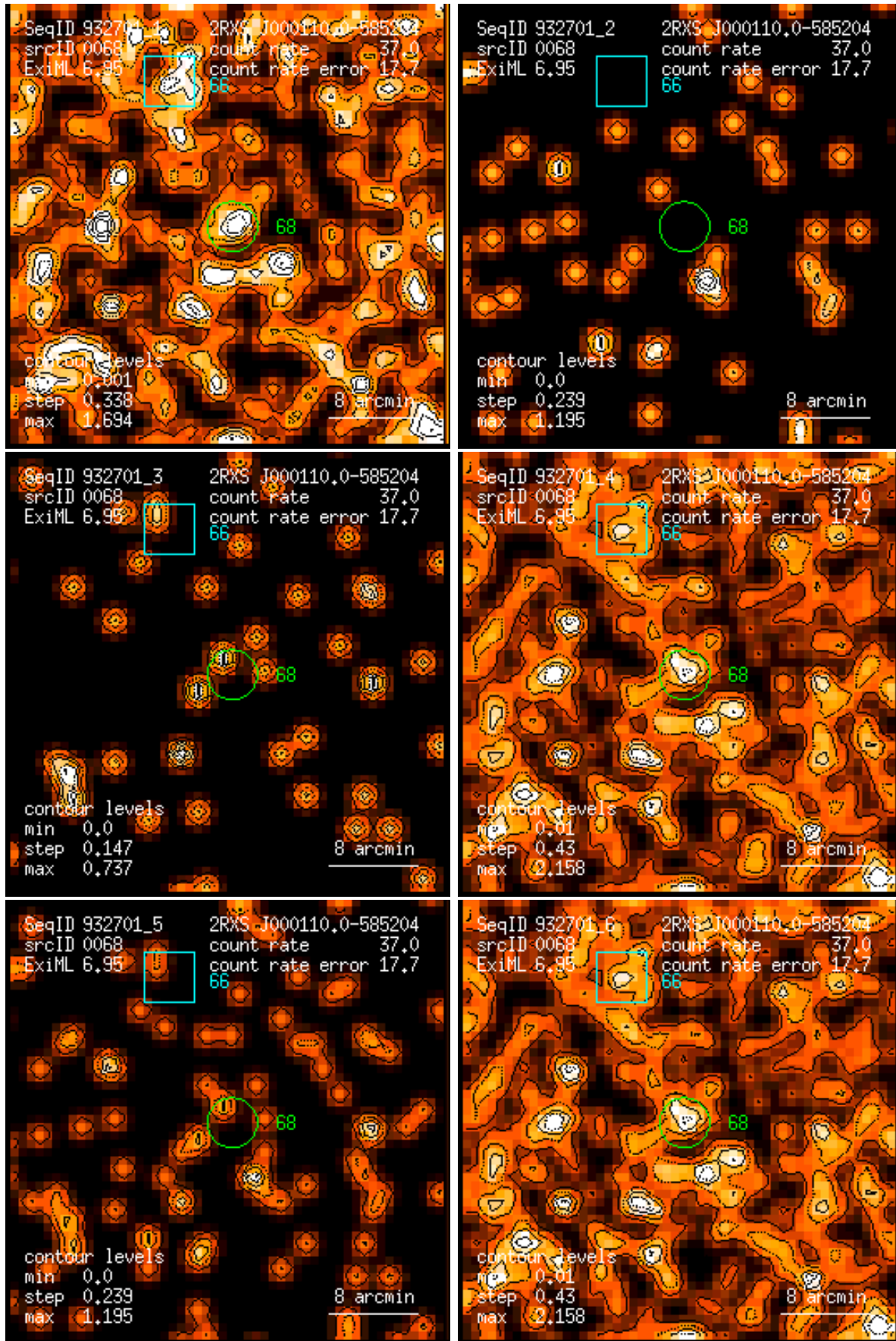
Figure 68: RASS 932701: detection 0068: band rate images, Gaussian filter: (1) PSPC channels 11 – 41, (2) 52 – 90, (3) 91 – 201, (4) 11 – 235, (5) 52 – 201, (6) 11 – 201. Broad band rates in counts/ks. Band rate contour levels in counts/ks/arcmin 2 .
