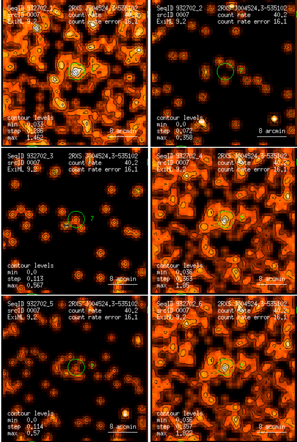
Figure 7: RASS 932702: detection 0007: band rate images, Gaussian filter: (1) PSPC channels 11 – 41, (2) 52 – 90, (3) 91 – 201, (4) 11 – 235, (5) 52 – 201, (6) 11 – 201. Broad band rates in counts/ks. Band rate contour levels in counts/ks/arcmin 2 .
