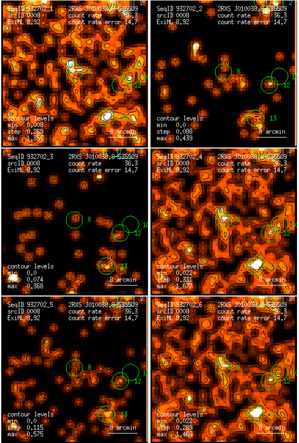
Figure 8: RASS 932702: detection 0008: band rate images, Gaussian filter: (1) PSPC channels 11 – 41, (2) 52 – 90, (3) 91 – 201, (4) 11 – 235, (5) 52 – 201, (6) 11 – 201. Broad band rates in counts/ks. Band rate contour levels in counts/ks/arcmin 2 .
