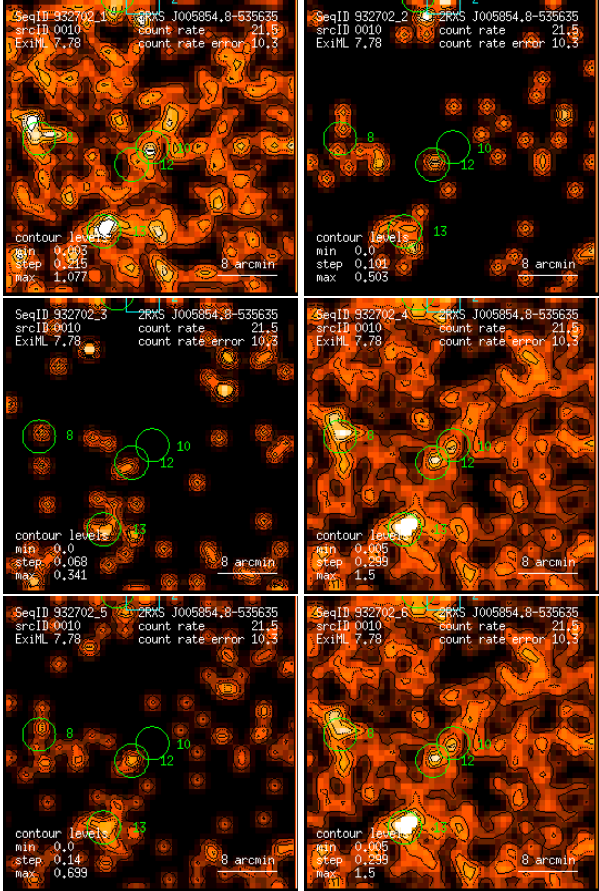
Figure 10: RASS 932702: detection 0010: band rate images, Gaussian filter: (1) PSPC channels 11 – 41, (2) 52 – 90, (3) 91 – 201, (4) 11 – 235, (5) 52 – 201, (6) 11 – 201. Broad band rates in counts/ks. Band rate contour levels in counts/ks/arcmin 2 .
