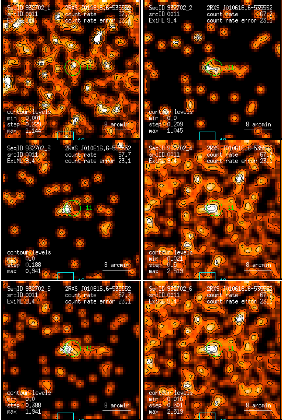
Figure 11: RASS 932702: detection 0011: band rate images, Gaussian filter: (1) PSPC channels 11 – 41, (2) 52 – 90, (3) 91 – 201, (4) 11 – 235, (5) 52 – 201, (6) 11 – 201. Broad band rates in counts/ks. Band rate contour levels in counts/ks/arcmin 2 .
