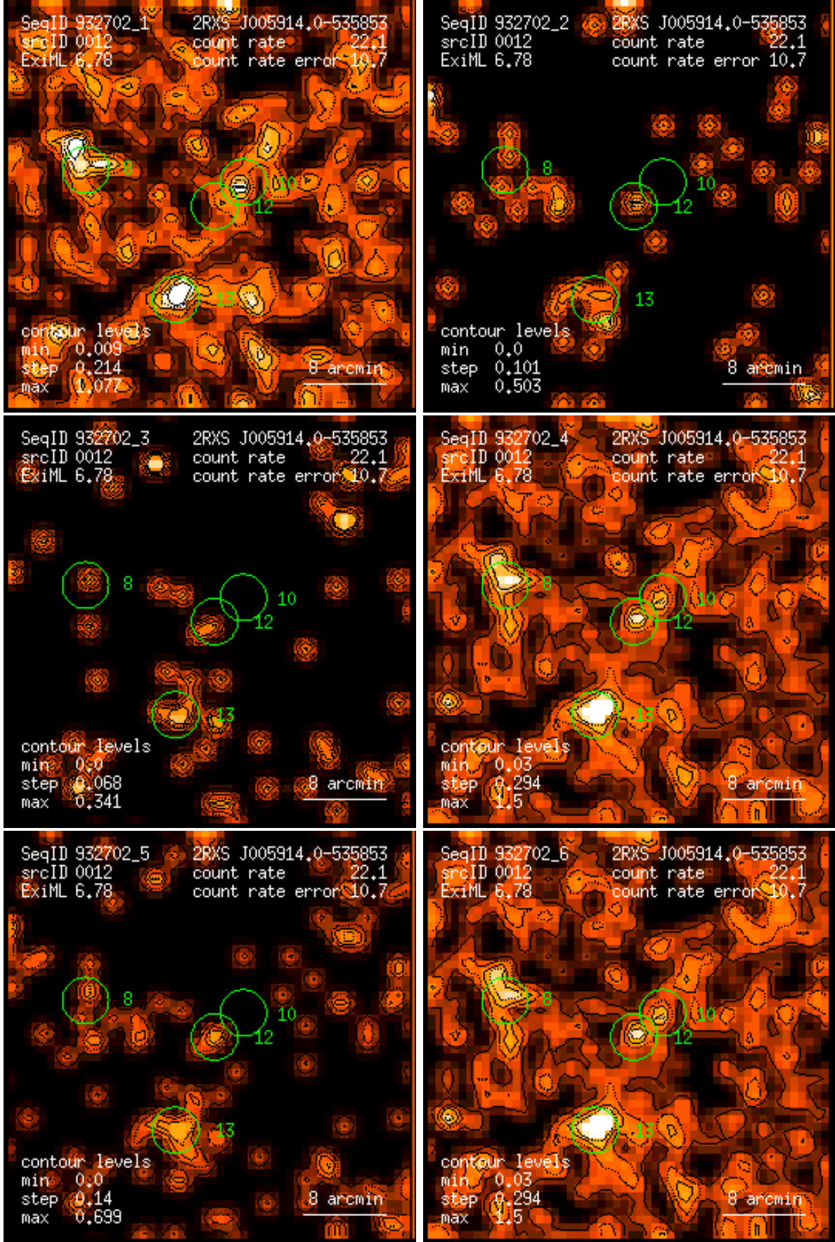
Figure 12: RASS 932702: detection 0012: band rate images, Gaussian filter: (1) PSPC channels 11 – 41, (2) 52 – 90, (3) 91 – 201, (4) 11 – 235, (5) 52 – 201, (6) 11 – 201. Broad band rates in counts/ks. Band rate contour levels in counts/ks/arcmin 2 .
