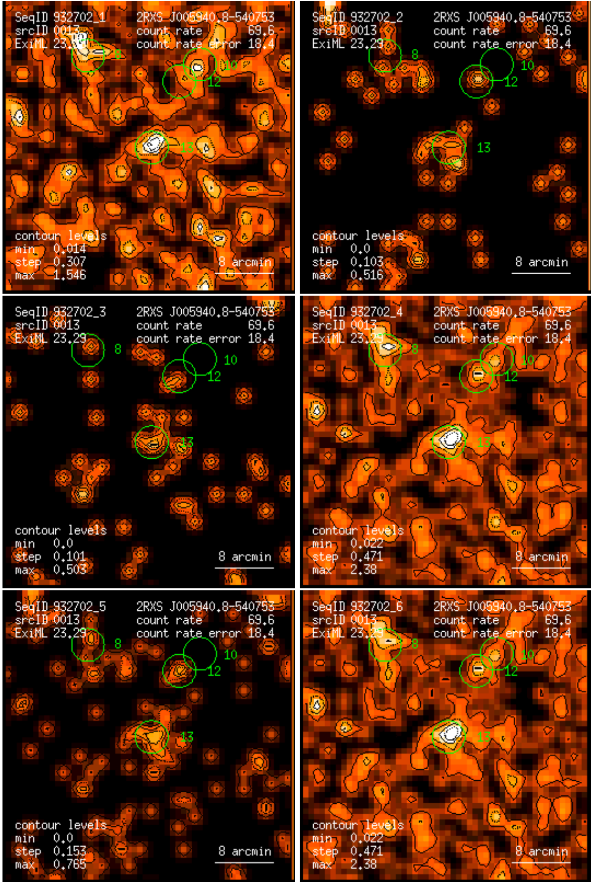
Figure 13: RASS 932702: detection 0013: band rate images, Gaussian filter: (1) PSPC channels 11 – 41, (2) 52 – 90, (3) 91 – 201, (4) 11 – 235, (5) 52 – 201, (6) 11 – 201. Broad band rates in counts/ks. Band rate contour levels in counts/ks/arcmin 2 .
