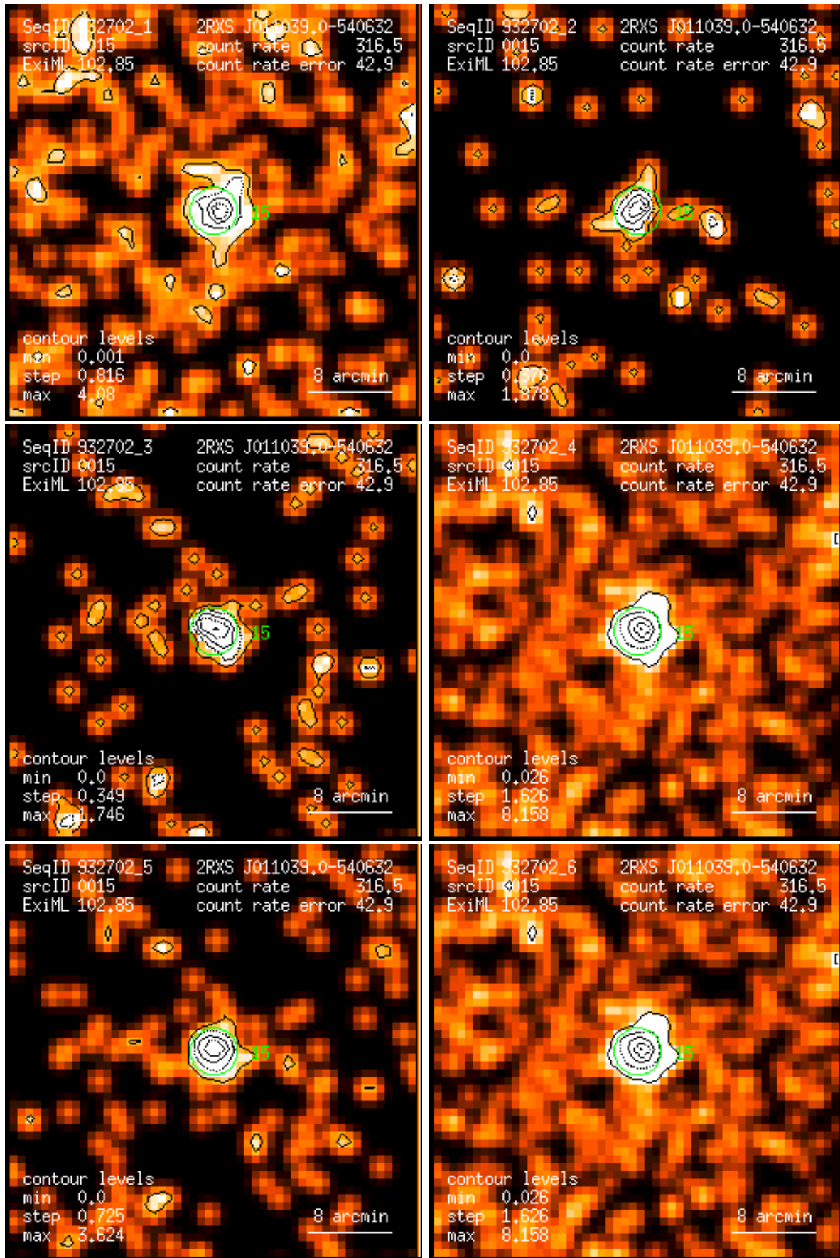
Figure 15: RASS 932702: detection 0015: band rate images, Gaussian filter: (1) PSPC channels 11 – 41, (2) 52 – 90, (3) 91 – 201, (4) 11 – 235, (5) 52 – 201, (6) 11 – 201. Broad band rates in counts/ks. Band rate contour levels in counts/ks/arcmin 2 .
