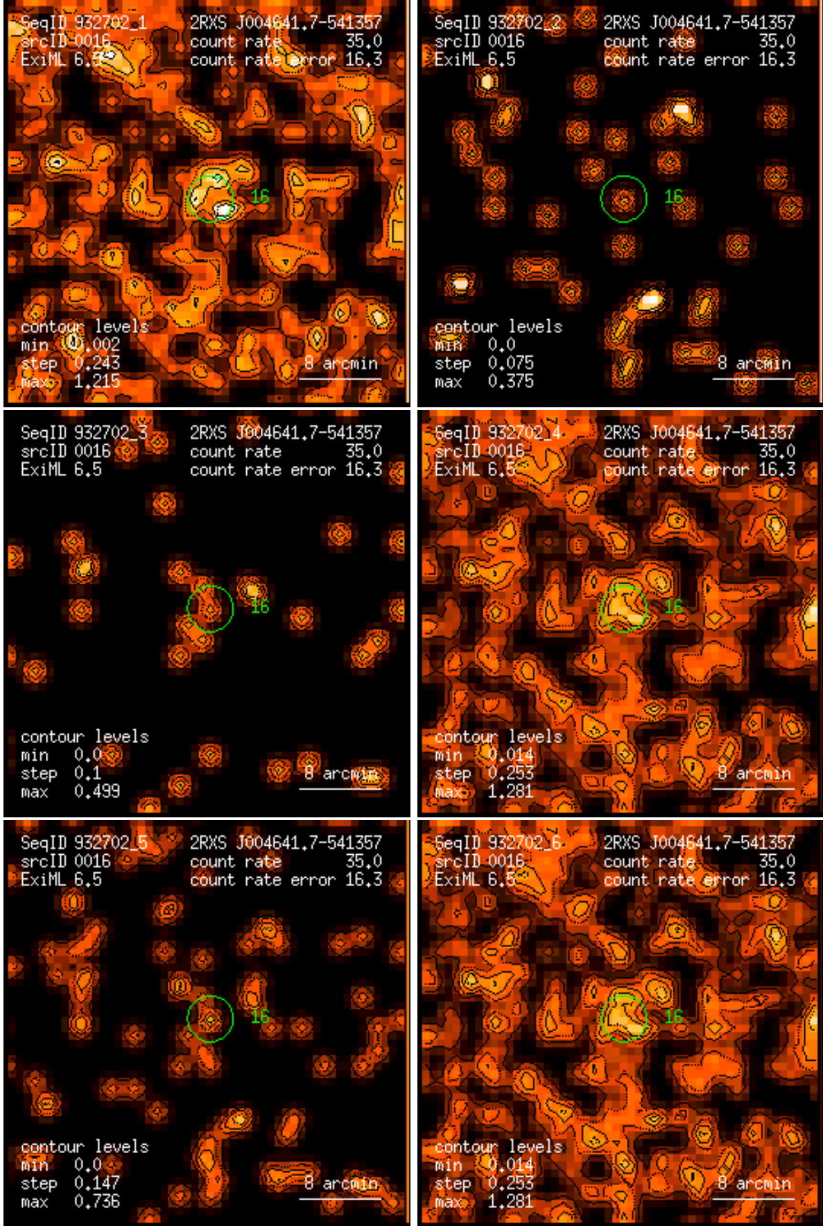
Figure 16: RASS 932702: detection 0016: band rate images, Gaussian filter: (1) PSPC channels 11 – 41, (2) 52 – 90, (3) 91 – 201, (4) 11 – 235, (5) 52 – 201, (6) 11 – 201. Broad band rates in counts/ks. Band rate contour levels in counts/ks/arcmin 2 .
