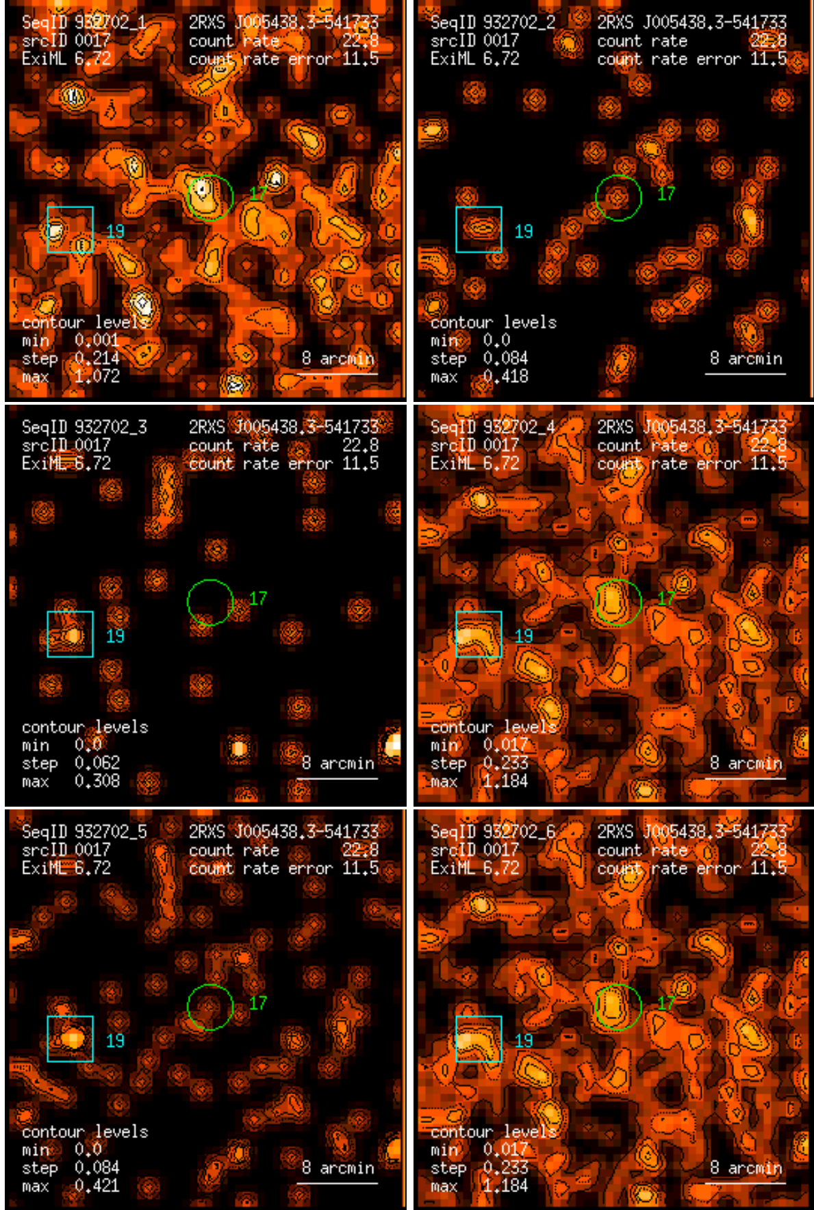
Figure 17: RASS 932702: detection 0017: band rate images, Gaussian filter: (1) PSPC channels 11 – 41, (2) 52 – 90, (3) 91 – 201, (4) 11 – 235, (5) 52 – 201, (6) 11 – 201. Broad band rates in counts/ks. Band rate contour levels in counts/ks/arcmin 2 .
