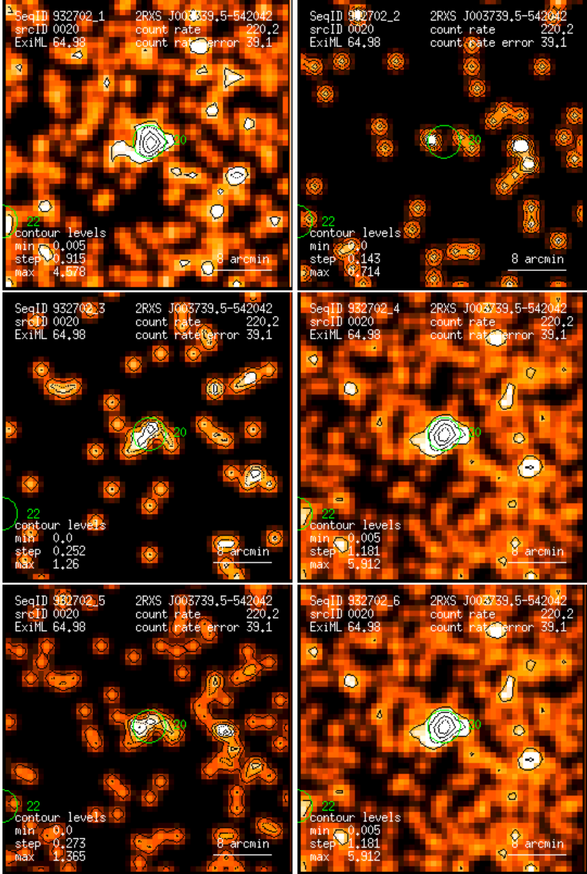
Figure 20: RASS 932702: detection 0020: band rate images, Gaussian filter: (1) PSPC channels 11 – 41, (2) 52 – 90, (3) 91 – 201, (4) 11 – 235, (5) 52 – 201, (6) 11 – 201. Broad band rates in counts/ks. Band rate contour levels in counts/ks/arcmin 2 .
