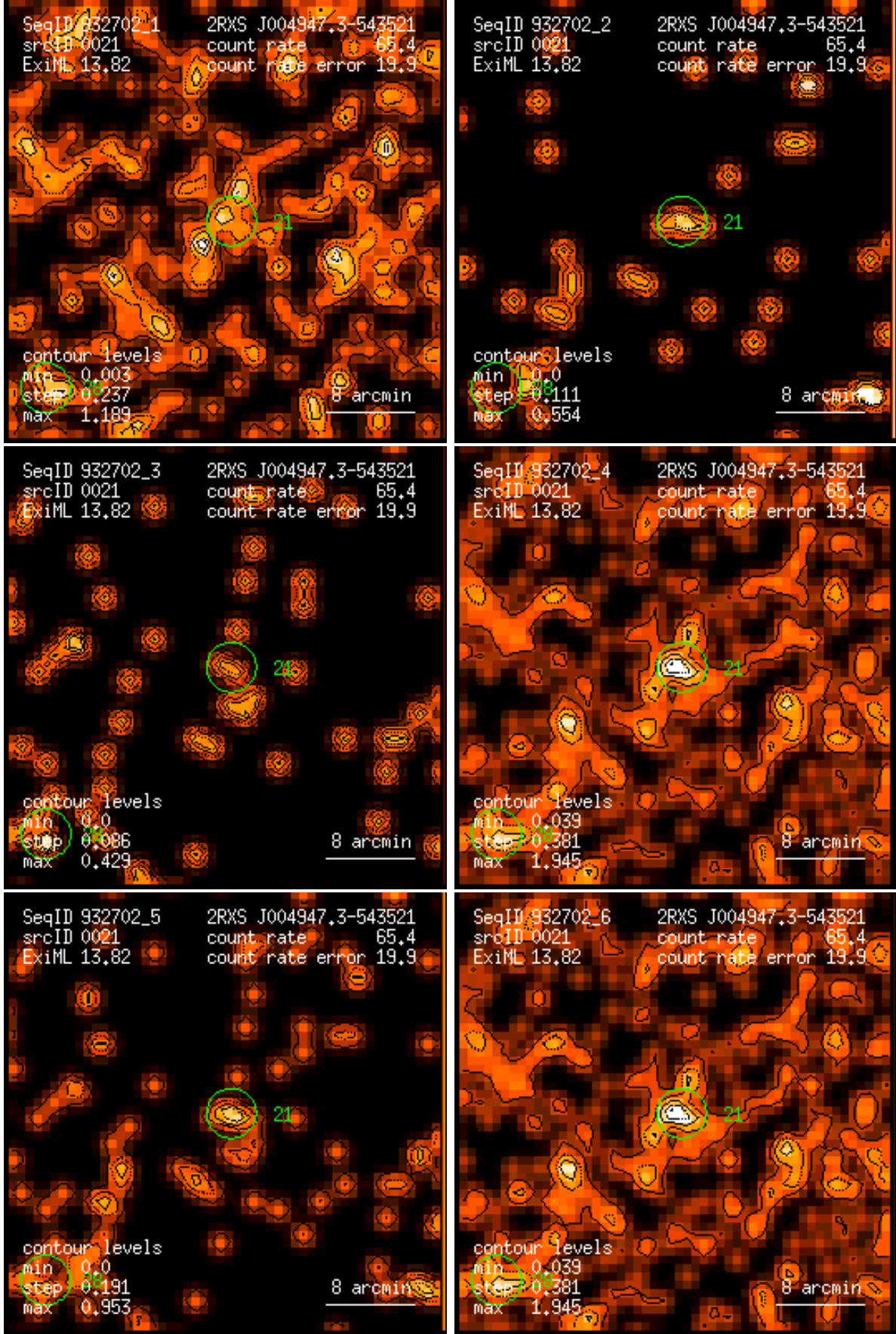
Figure 21: RASS 932702: detection 0021: band rate images, Gaussian filter: (1) PSPC channels 11 – 41, (2) 52 – 90, (3) 91 – 201, (4) 11 – 235, (5) 52 – 201, (6) 11 – 201. Broad band rates in counts/ks. Band rate contour levels in counts/ks/arcmin 2 .
