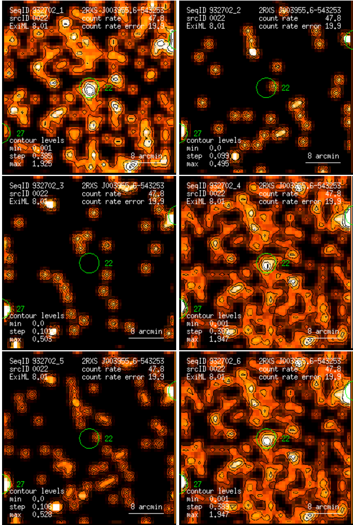
Figure 22: RASS 932702: detection 0022: band rate images, Gaussian filter: (1) PSPC channels 11 – 41, (2) 52 – 90, (3) 91 – 201, (4) 11 – 235, (5) 52 – 201, (6) 11 – 201. Broad band rates in counts/ks. Band rate contour levels in counts/ks/arcmin 2 .
