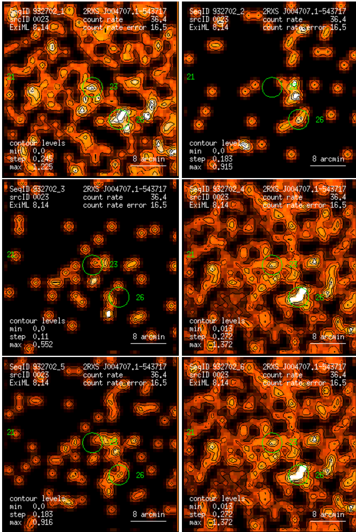
Figure 23: RASS 932702: detection 0023: band rate images, Gaussian filter: (1) PSPC channels 11 – 41, (2) 52 – 90, (3) 91 – 201, (4) 11 – 235, (5) 52 – 201, (6) 11 – 201. Broad band rates in counts/ks. Band rate contour levels in counts/ks/arcmin 2 .
