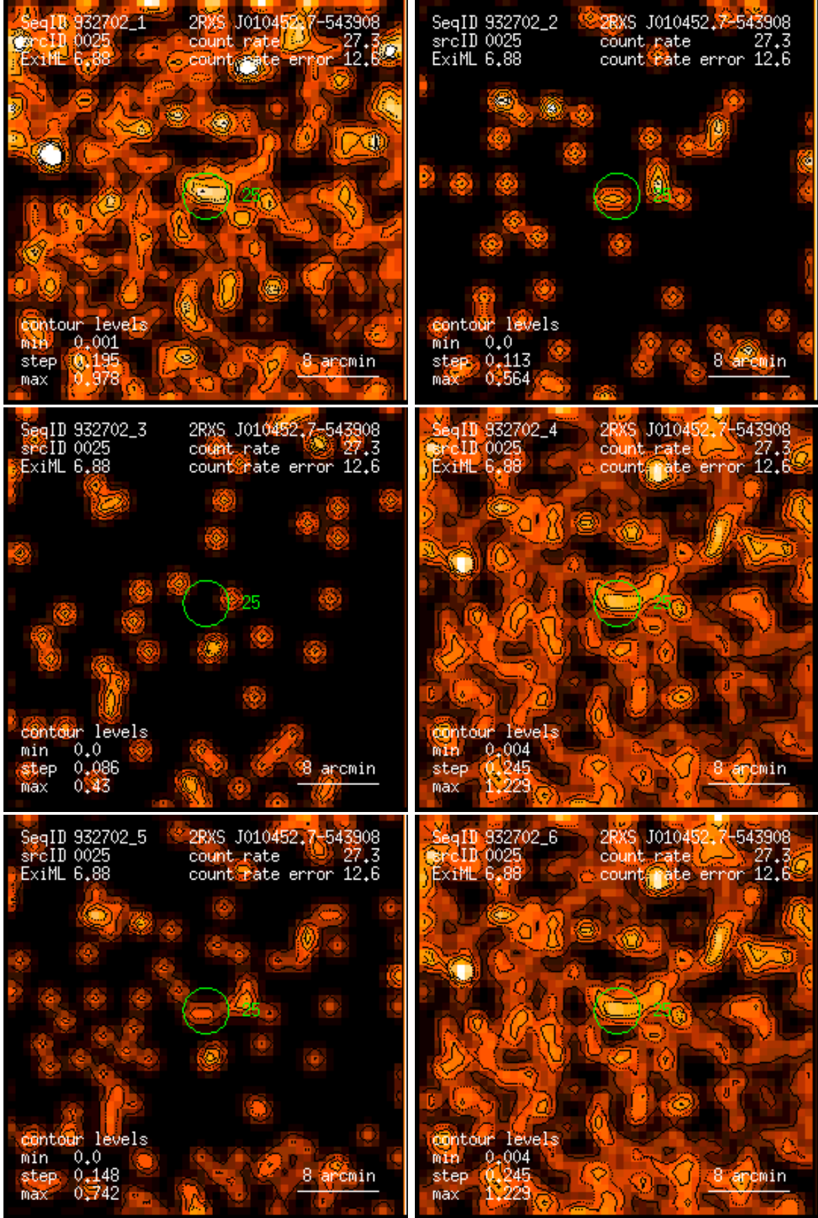
Figure 25: RASS 932702: detection 0025: band rate images, Gaussian filter: (1) PSPC channels 11 – 41, (2) 52 – 90, (3) 91 – 201, (4) 11 – 235, (5) 52 – 201, (6) 11 – 201. Broad band rates in counts/ks. Band rate contour levels in counts/ks/arcmin 2 .
