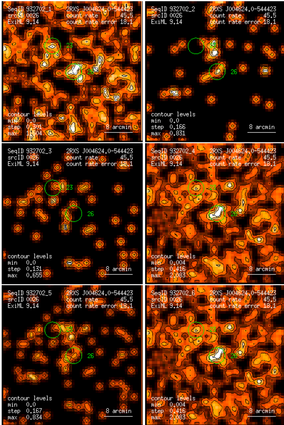
Figure 26: RASS 932702: detection 0026: band rate images, Gaussian filter: (1) PSPC channels 11 – 41, (2) 52 – 90, (3) 91 – 201, (4) 11 – 235, (5) 52 – 201, (6) 11 – 201. Broad band rates in counts/ks. Band rate contour levels in counts/ks/arcmin 2 .
