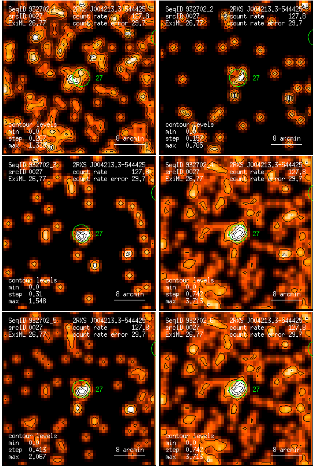
Figure 27: RASS 932702: detection 0027: band rate images, Gaussian filter: (1) PSPC channels 11 – 41, (2) 52 – 90, (3) 91 – 201, (4) 11 – 235, (5) 52 – 201, (6) 11 – 201. Broad band rates in counts/ks. Band rate contour levels in counts/ks/arcmin 2 .
