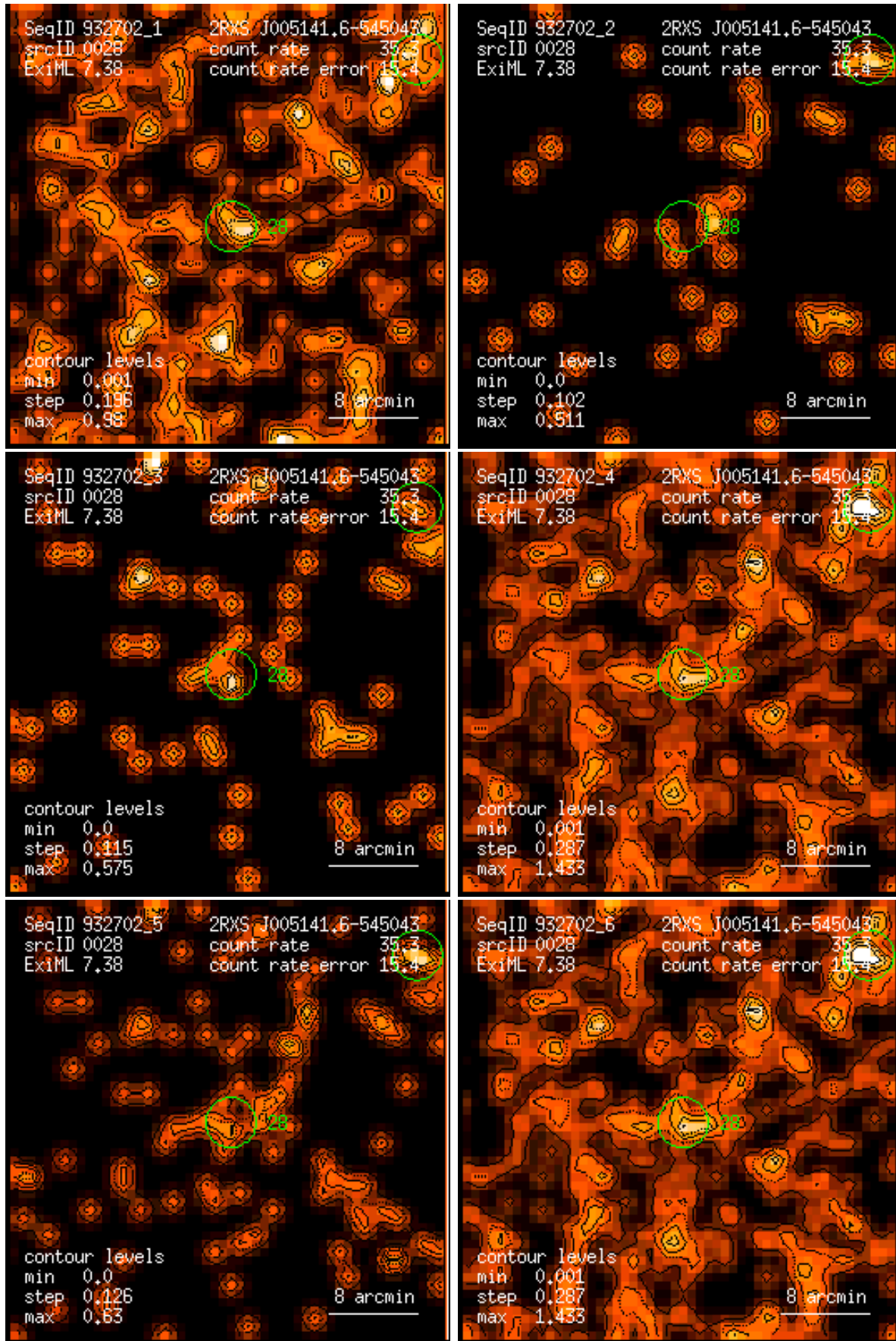
Figure 28: RASS 932702: detection 0028: band rate images, Gaussian filter: (1) PSPC channels 11 – 41, (2) 52 – 90, (3) 91 – 201, (4) 11 – 235, (5) 52 – 201, (6) 11 – 201. Broad band rates in counts/ks. Band rate contour levels in counts/ks/arcmin 2 .
