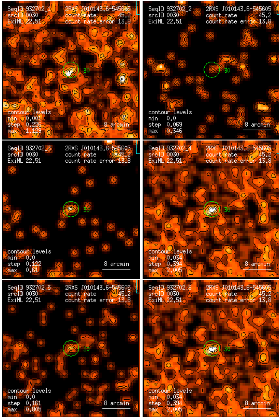
Figure 30: RASS 932702: detection 0030: band rate images, Gaussian filter: (1) PSPC channels 11 – 41, (2) 52 – 90, (3) 91 – 201, (4) 11 – 235, (5) 52 – 201, (6) 11 – 201. Broad band rates in counts/ks. Band rate contour levels in counts/ks/arcmin 2 .
