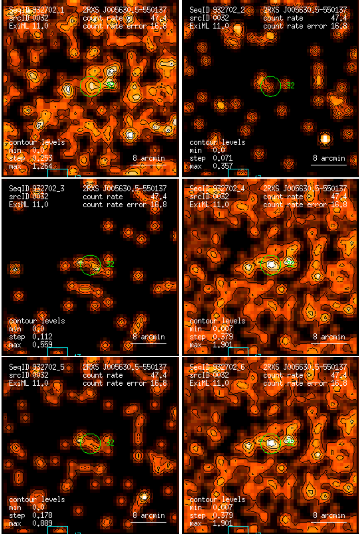
Figure 32: RASS 932702: detection 0032: band rate images, Gaussian filter: (1) PSPC channels 11 – 41, (2) 52 – 90, (3) 91 – 201, (4) 11 – 235, (5) 52 – 201, (6) 11 – 201. Broad band rates in counts/ks. Band rate contour levels in counts/ks/arcmin 2 .
