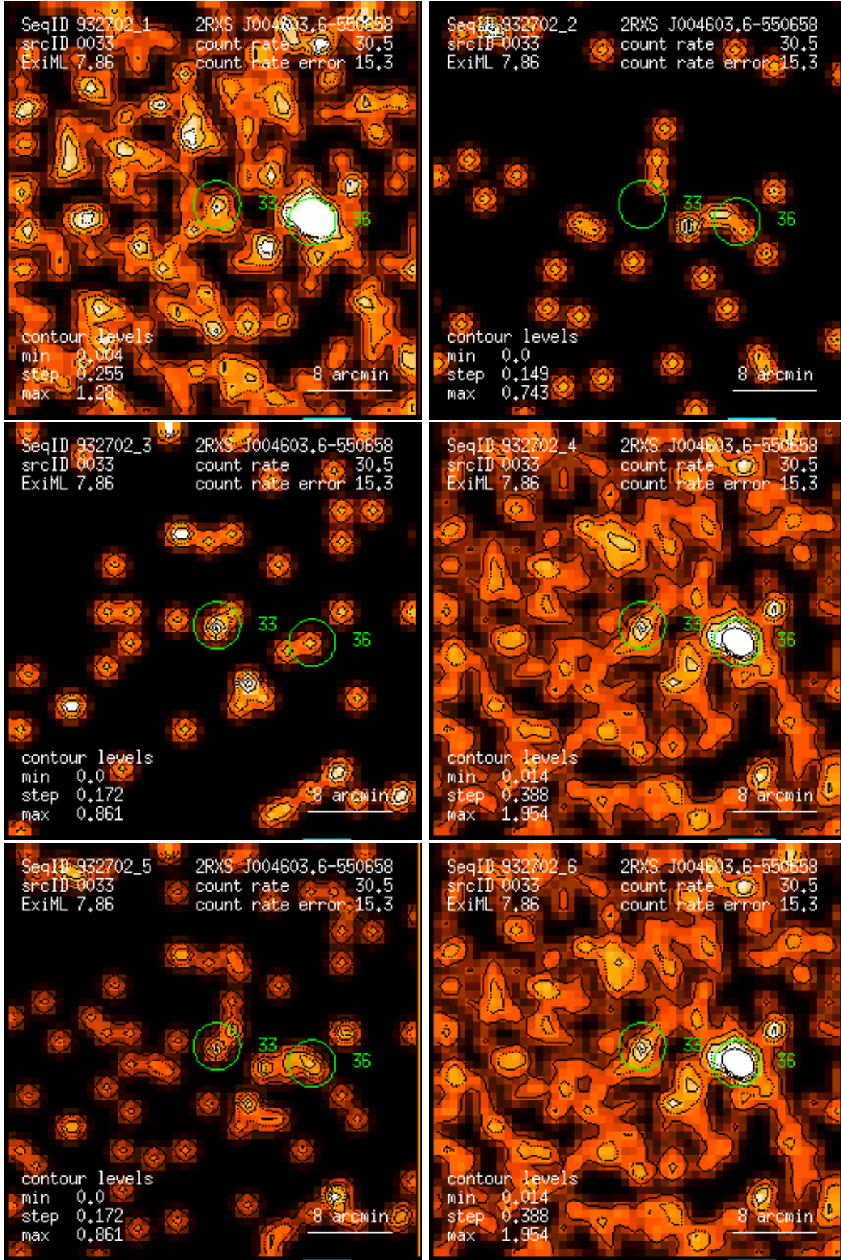
Figure 33: RASS 932702: detection 0033: band rate images, Gaussian filter: (1) PSPC channels 11 – 41, (2) 52 – 90, (3) 91 – 201, (4) 11 – 235, (5) 52 – 201, (6) 11 – 201. Broad band rates in counts/ks. Band rate contour levels in counts/ks/arcmin 2 .
