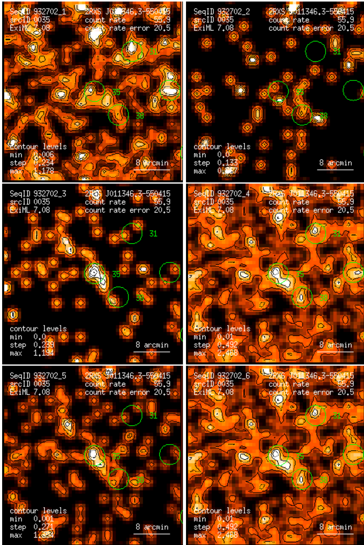
Figure 35: RASS 932702: detection 0035: band rate images, Gaussian filter: (1) PSPC channels 11 – 41, (2) 52 – 90, (3) 91 – 201, (4) 11 – 235, (5) 52 – 201, (6) 11 – 201. Broad band rates in counts/ks. Band rate contour levels in counts/ks/arcmin 2 .
