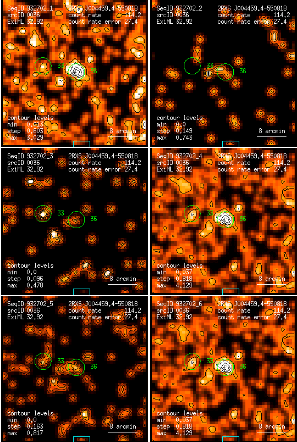
Figure 36: RASS 932702: detection 0036: band rate images, Gaussian filter: (1) PSPC channels 11 – 41, (2) 52 – 90, (3) 91 – 201, (4) 11 – 235, (5) 52 – 201, (6) 11 – 201. Broad band rates in counts/ks. Band rate contour levels in counts/ks/arcmin 2 .
