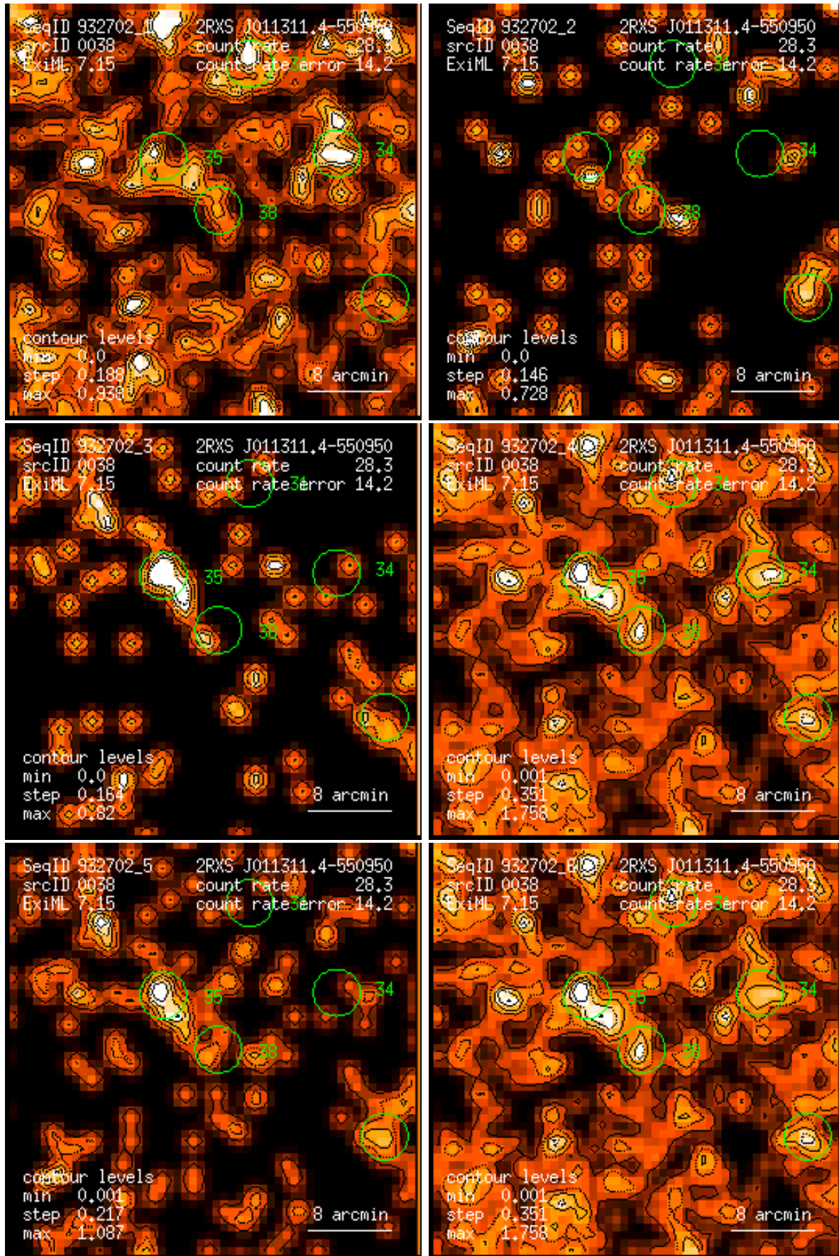
Figure 38: RASS 932702: detection 0038: band rate images, Gaussian filter: (1) PSPC channels 11 – 41, (2) 52 – 90, (3) 91 – 201, (4) 11 – 235, (5) 52 – 201, (6) 11 – 201. Broad band rates in counts/ks. Band rate contour levels in counts/ks/arcmin 2 .
