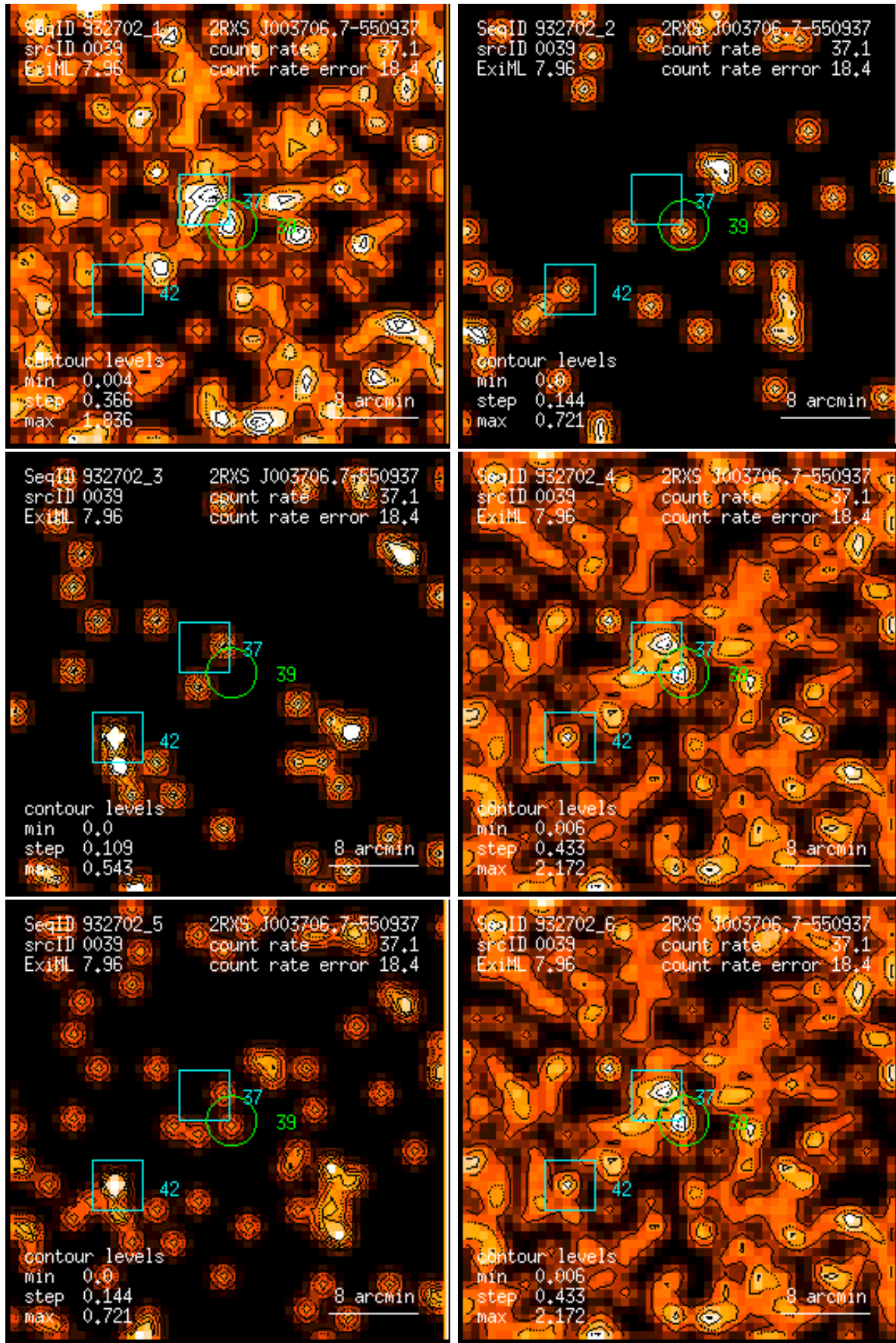
Figure 39: RASS 932702: detection 0039: band rate images, Gaussian filter: (1) PSPC channels 11 – 41, (2) 52 – 90, (3) 91 – 201, (4) 11 – 235, (5) 52 – 201, (6) 11 – 201. Broad band rates in counts/ks. Band rate contour levels in counts/ks/arcmin 2 .
