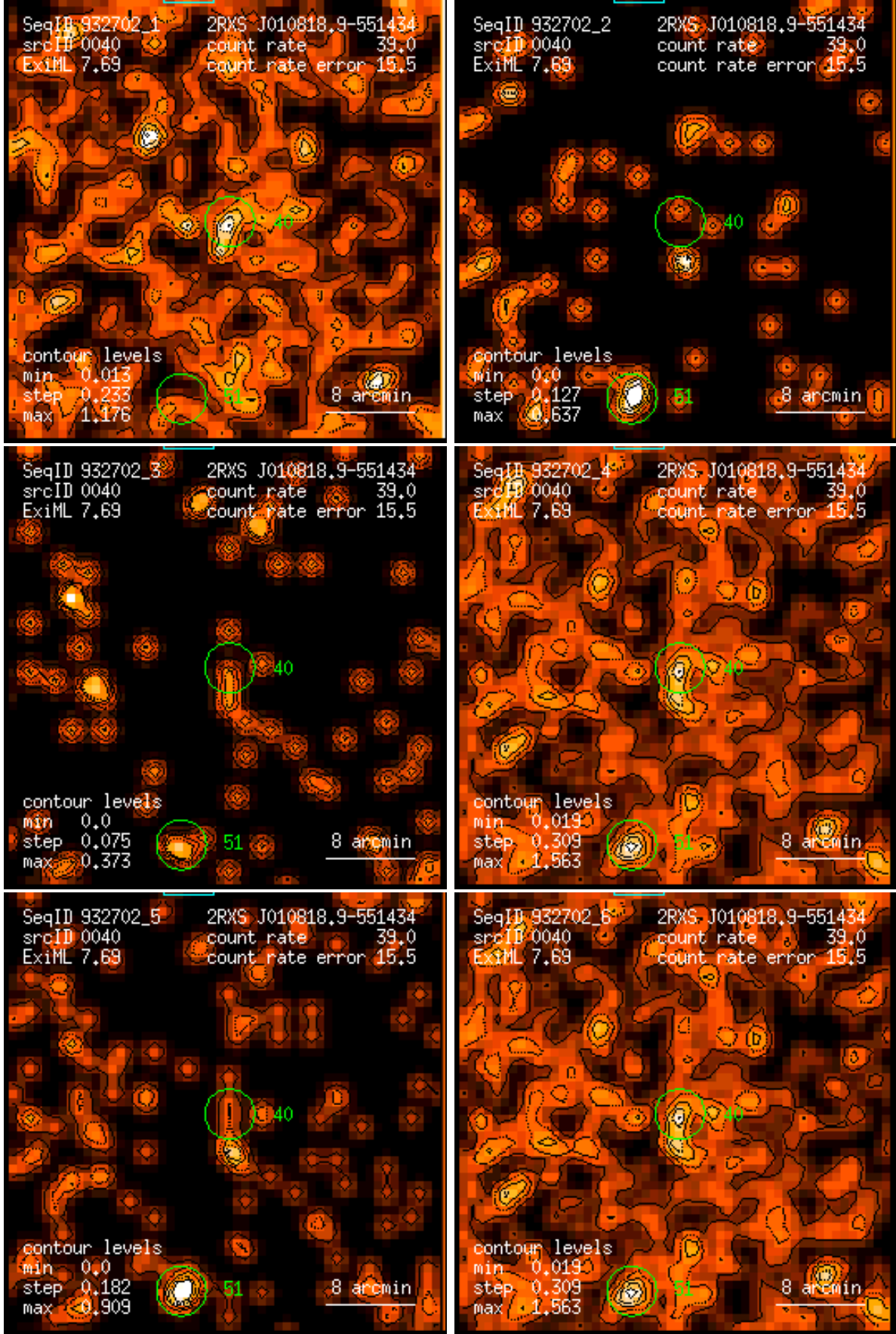
Figure 40: RASS 932702: detection 0040: band rate images, Gaussian filter: (1) PSPC channels 11 – 41, (2) 52 – 90, (3) 91 – 201, (4) 11 – 235, (5) 52 – 201, (6) 11 – 201. Broad band rates in counts/ks. Band rate contour levels in counts/ks/arcmin 2 .
