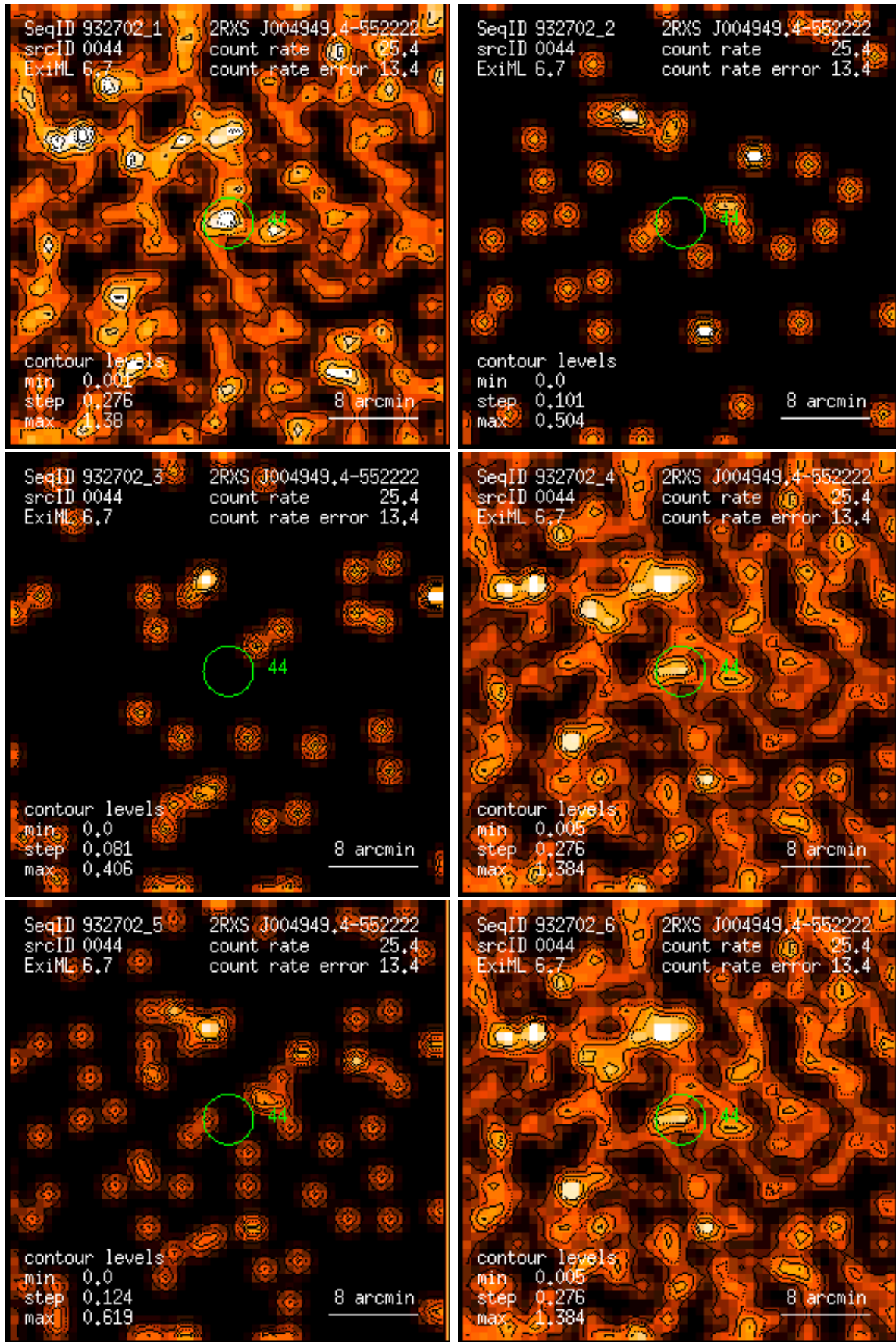
Figure 44: RASS 932702: detection 0044: band rate images, Gaussian filter: (1) PSPC channels 11 – 41, (2) 52 – 90, (3) 91 – 201, (4) 11 – 235, (5) 52 – 201, (6) 11 – 201. Broad band rates in counts/ks. Band rate contour levels in counts/ks/arcmin 2 .
