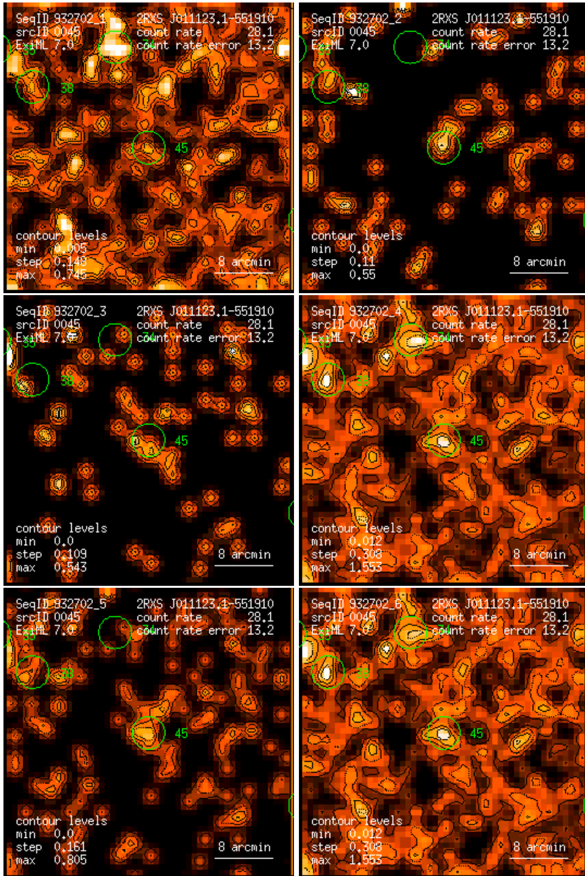
Figure 45: RASS 932702: detection 0045: band rate images, Gaussian filter: (1) PSPC channels 11 – 41, (2) 52 – 90, (3) 91 – 201, (4) 11 – 235, (5) 52 – 201, (6) 11 – 201. Broad band rates in counts/ks. Band rate contour levels in counts/ks/arcmin 2 .
