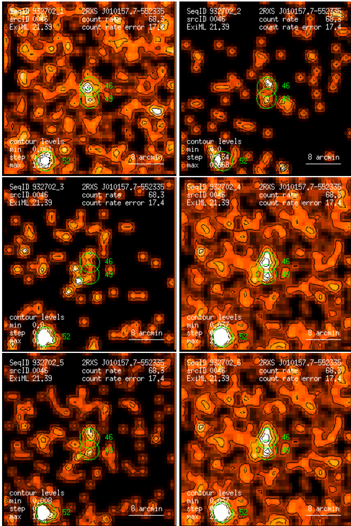
Figure 46: RASS 932702: detection 0046: band rate images, Gaussian filter: (1) PSPC channels 11 – 41, (2) 52 – 90, (3) 91 – 201, (4) 11 – 235, (5) 52 – 201, (6) 11 – 201. Broad band rates in counts/ks. Band rate contour levels in counts/ks/arcmin 2 .
