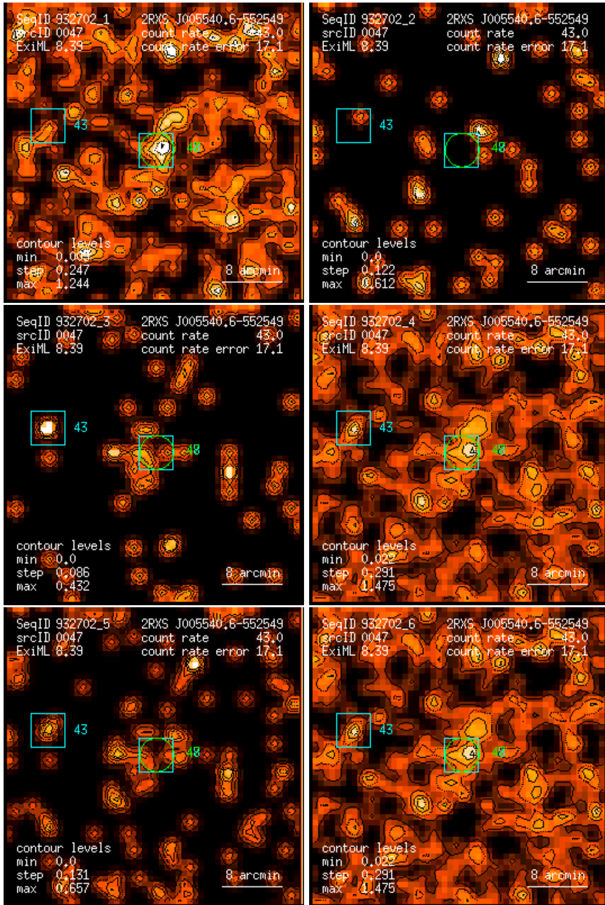
Figure 47: RASS 932702: detection 0047: band rate images, Gaussian filter: (1) PSPC channels 11 – 41, (2) 52 – 90, (3) 91 – 201, (4) 11 – 235, (5) 52 – 201, (6) 11 – 201. Broad band rates in counts/ks. Band rate contour levels in counts/ks/arcmin 2 .
