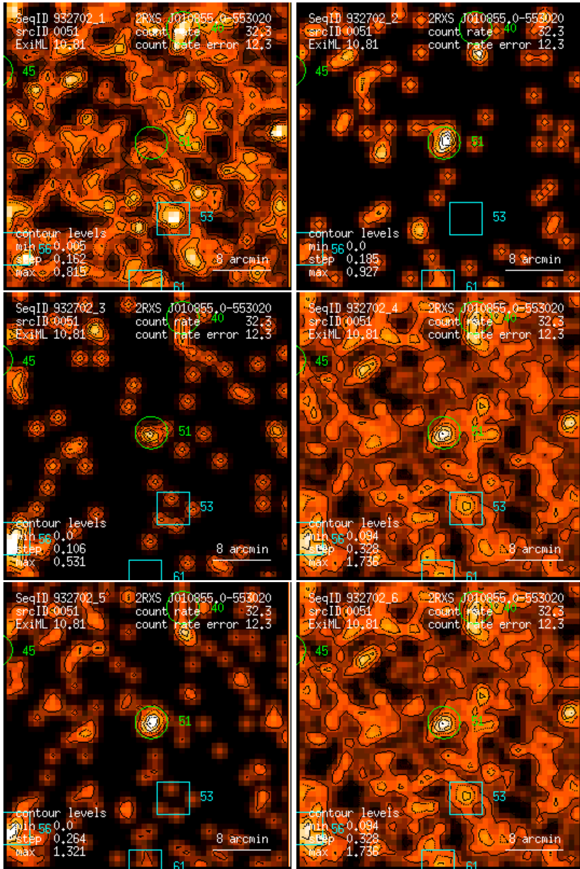
Figure 51: RASS 932702: detection 0051: band rate images, Gaussian filter: (1) PSPC channels 11 – 41, (2) 52 – 90, (3) 91 – 201, (4) 11 – 235, (5) 52 – 201, (6) 11 – 201. Broad band rates in counts/ks. Band rate contour levels in counts/ks/arcmin 2 .
