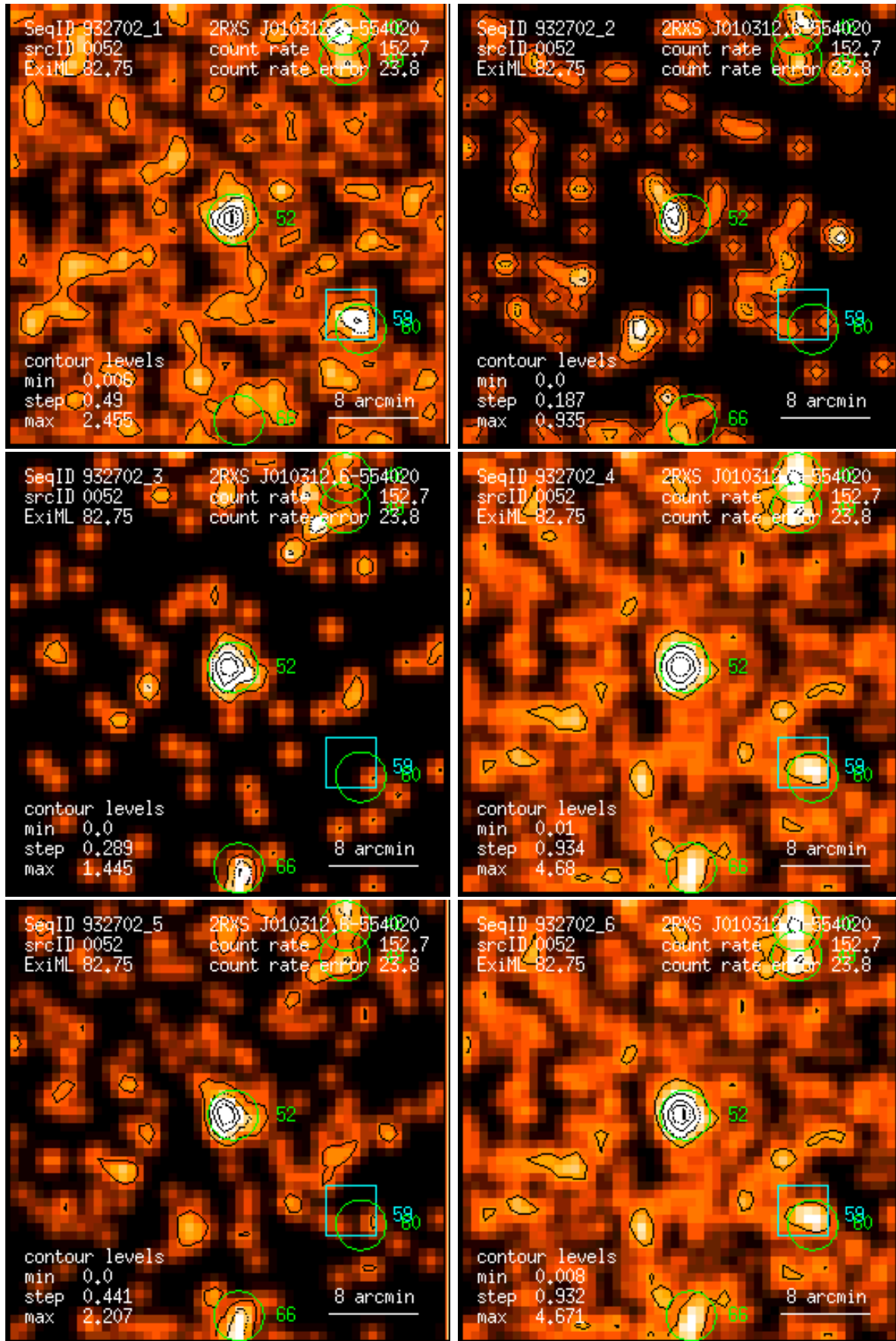
Figure 52: RASS 932702: detection 0052: band rate images, Gaussian filter: (1) PSPC channels 11 – 41, (2) 52 – 90, (3) 91 – 201, (4) 11 – 235, (5) 52 – 201, (6) 11 – 201. Broad band rates in counts/ks. Band rate contour levels in counts/ks/arcmin 2 .
