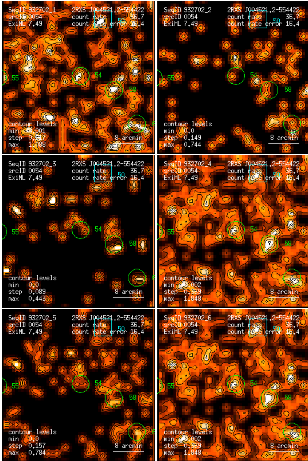
Figure 54: RASS 932702: detection 0054: band rate images, Gaussian filter: (1) PSPC channels 11 – 41, (2) 52 – 90, (3) 91 – 201, (4) 11 – 235, (5) 52 – 201, (6) 11 – 201. Broad band rates in counts/ks. Band rate contour levels in counts/ks/arcmin 2 .
