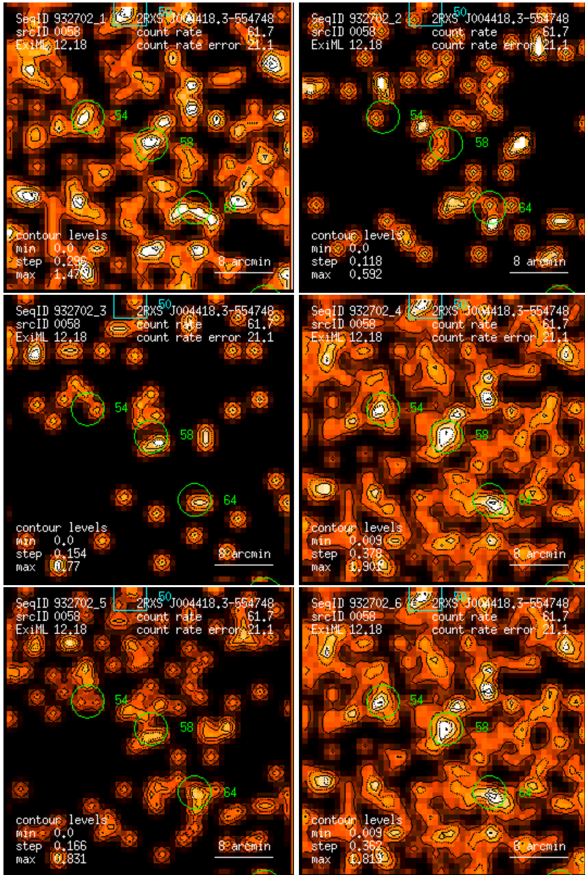
Figure 58: RASS 932702: detection 0058: band rate images, Gaussian filter: (1) PSPC channels 11 – 41, (2) 52 – 90, (3) 91 – 201, (4) 11 – 235, (5) 52 – 201, (6) 11 – 201. Broad band rates in counts/ks. Band rate contour levels in counts/ks/arcmin 2 .
