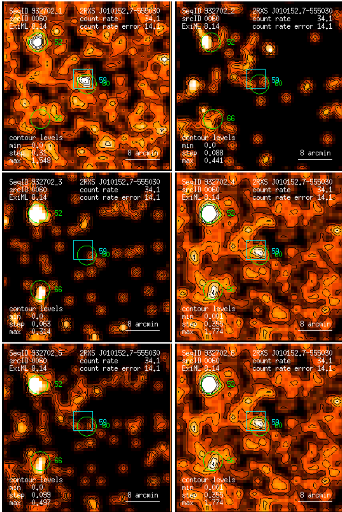
Figure 60: RASS 932702: detection 0060: band rate images, Gaussian filter: (1) PSPC channels 11 – 41, (2) 52 – 90, (3) 91 – 201, (4) 11 – 235, (5) 52 – 201, (6) 11 – 201. Broad band rates in counts/ks. Band rate contour levels in counts/ks/arcmin 2 .
