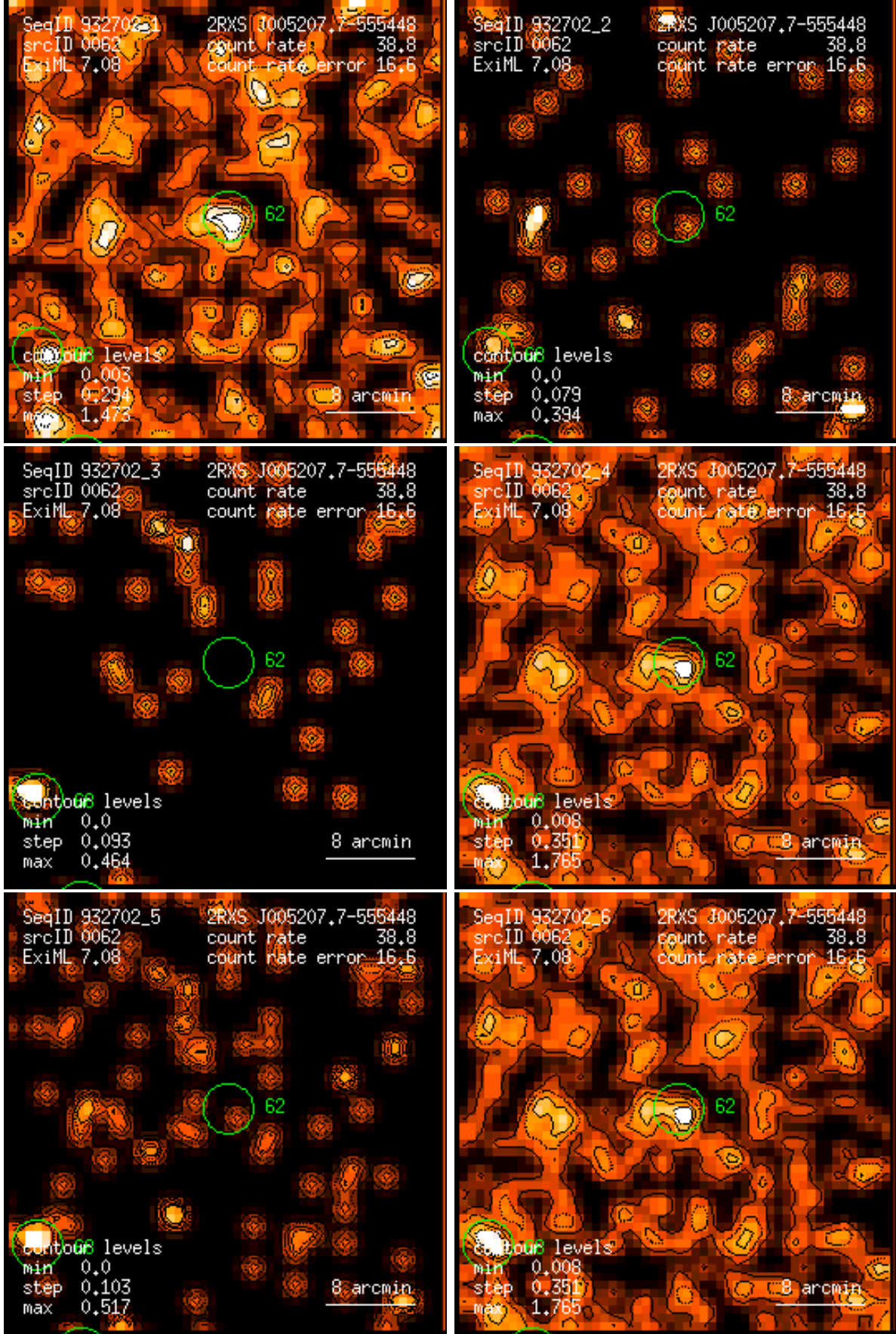
Figure 62: RASS 932702: detection 0062: band rate images, Gaussian filter: (1) PSPC channels 11 – 41, (2) 52 – 90, (3) 91 – 201, (4) 11 – 235, (5) 52 – 201, (6) 11 – 201. Broad band rates in counts/ks. Band rate contour levels in counts/ks/arcmin 2 .
