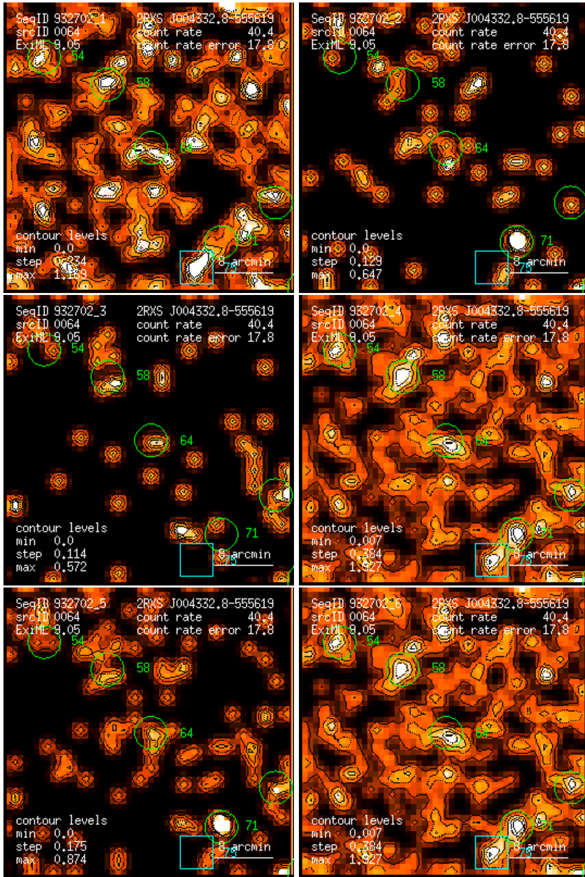
Figure 64: RASS 932702: detection 0064: band rate images, Gaussian filter: (1) PSPC channels 11 – 41, (2) 52 – 90, (3) 91 – 201, (4) 11 – 235, (5) 52 – 201, (6) 11 – 201. Broad band rates in counts/ks. Band rate contour levels in counts/ks/arcmin 2 .
