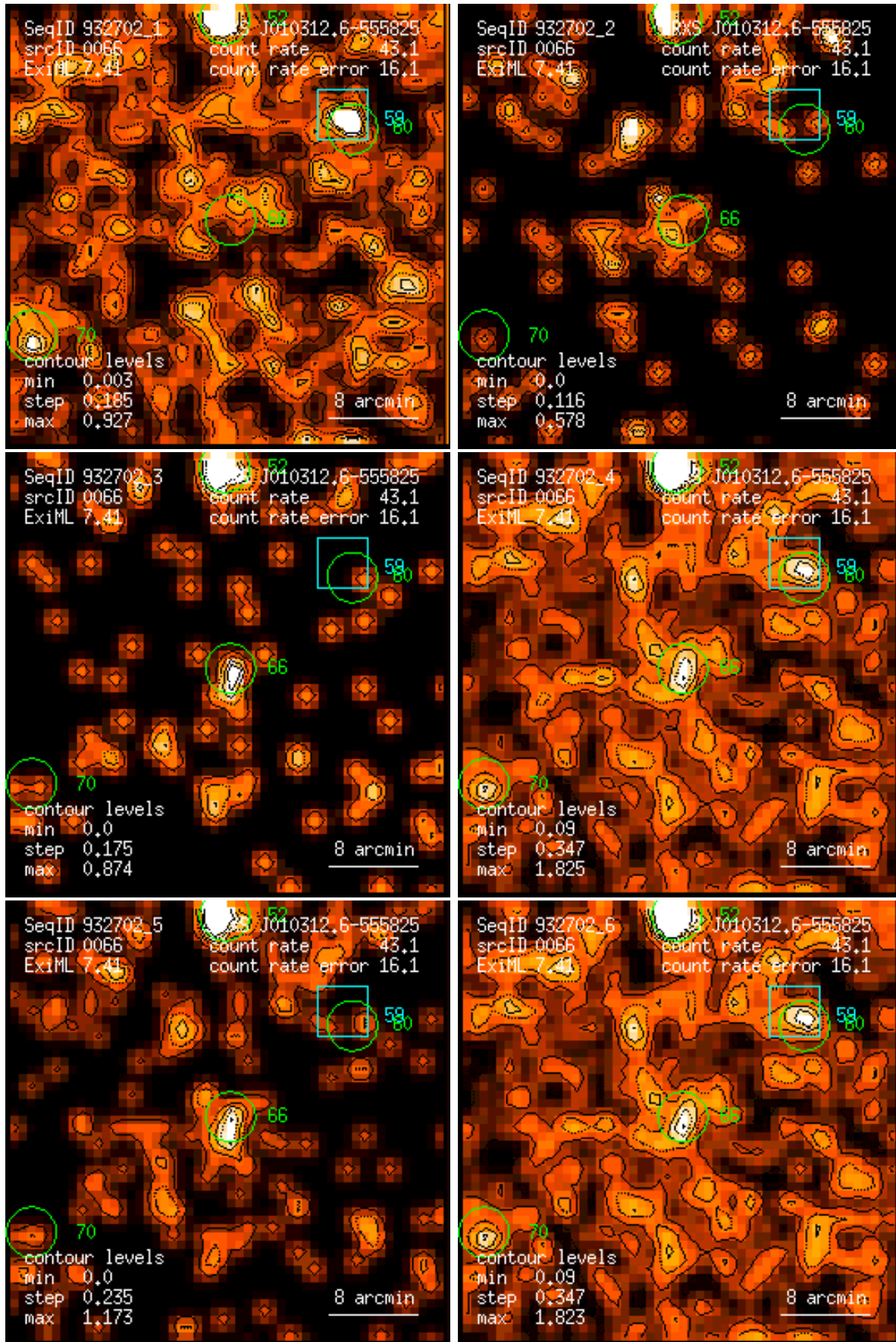
Figure 66: RASS 932702: detection 0066: band rate images, Gaussian filter: (1) PSPC channels 11 – 41, (2) 52 – 90, (3) 91 – 201, (4) 11 – 235, (5) 52 – 201, (6) 11 – 201. Broad band rates in counts/ks. Band rate contour levels in counts/ks/arcmin 2 .
