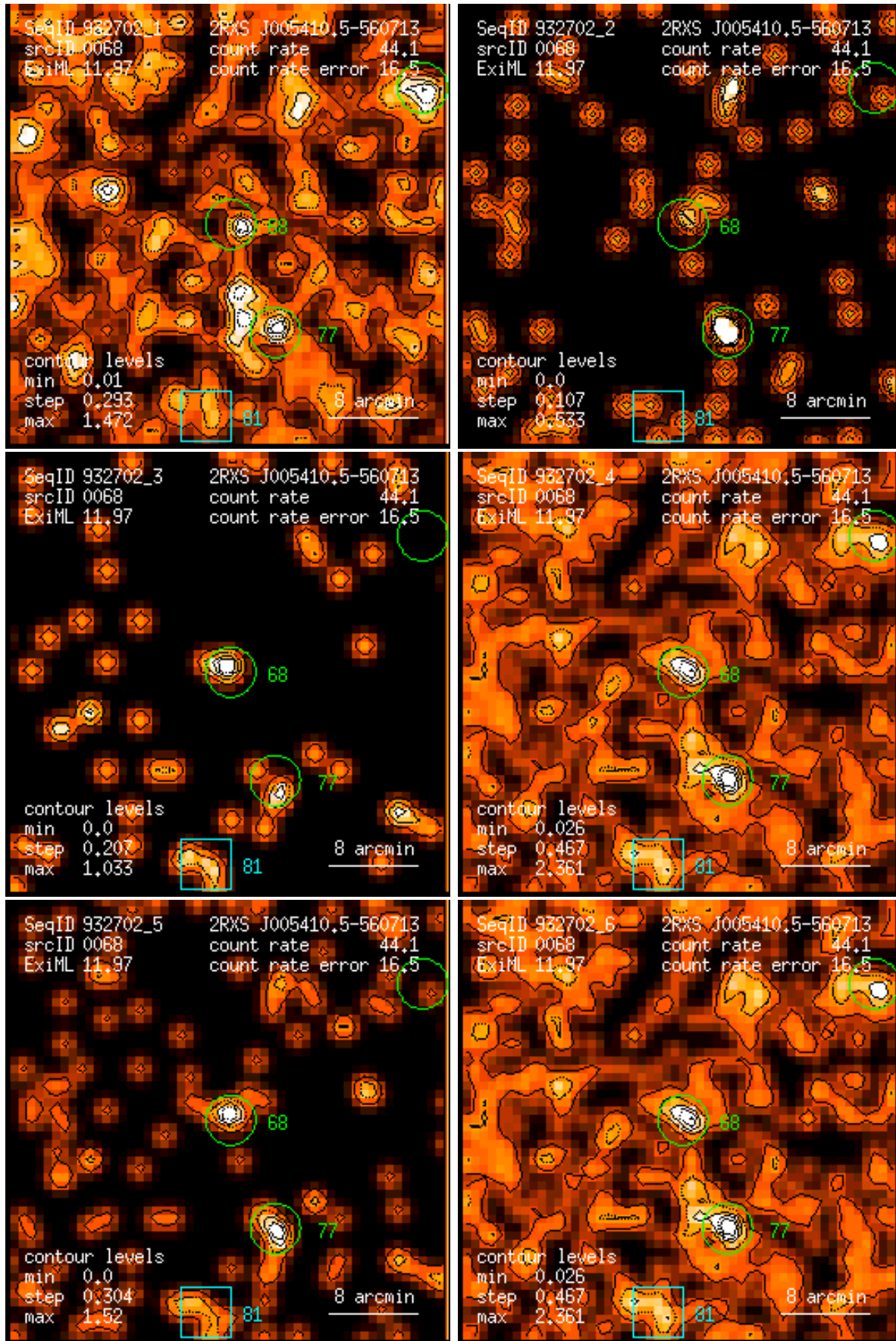
Figure 68: RASS 932702: detection 0068: band rate images, Gaussian filter: (1) PSPC channels 11 – 41, (2) 52 – 90, (3) 91 – 201, (4) 11 – 235, (5) 52 – 201, (6) 11 – 201. Broad band rates in counts/ks. Band rate contour levels in counts/ks/arcmin 2 .
