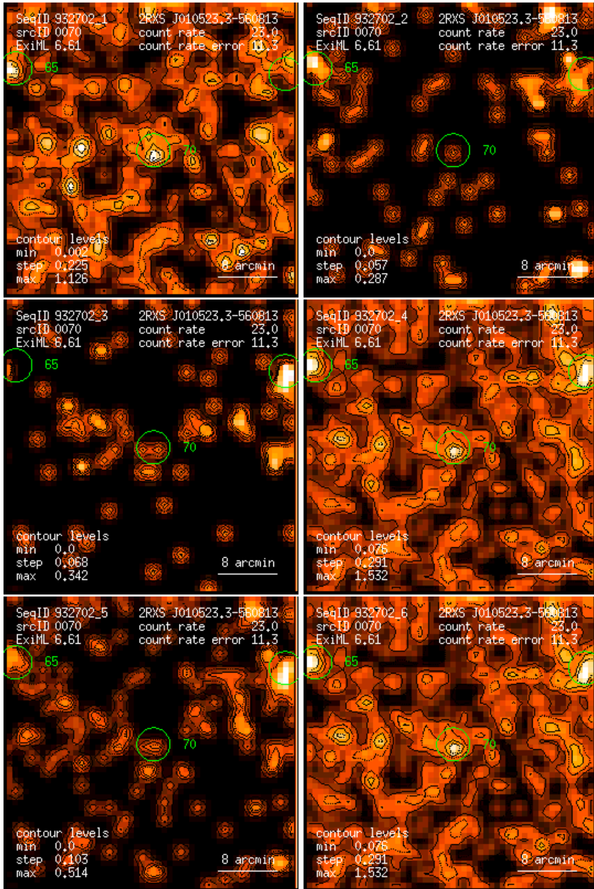
Figure 70: RASS 932702: detection 0070: band rate images, Gaussian filter: (1) PSPC channels 11 – 41, (2) 52 – 90, (3) 91 – 201, (4) 11 – 235, (5) 52 – 201, (6) 11 – 201. Broad band rates in counts/ks. Band rate contour levels in counts/ks/arcmin 2 .
