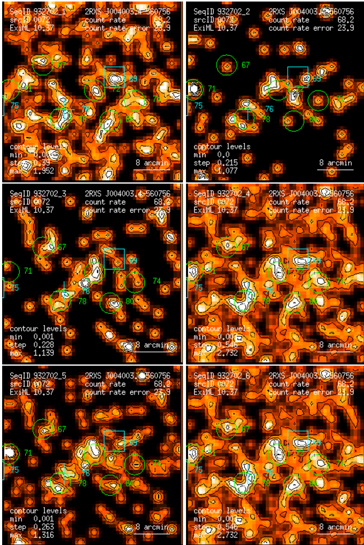
Figure 72: RASS 932702: detection 0072: band rate images, Gaussian filter: (1) PSPC channels 11 – 41, (2) 52 – 90, (3) 91 – 201, (4) 11 – 235, (5) 52 – 201, (6) 11 – 201. Broad band rates in counts/ks. Band rate contour levels in counts/ks/arcmin 2 .
