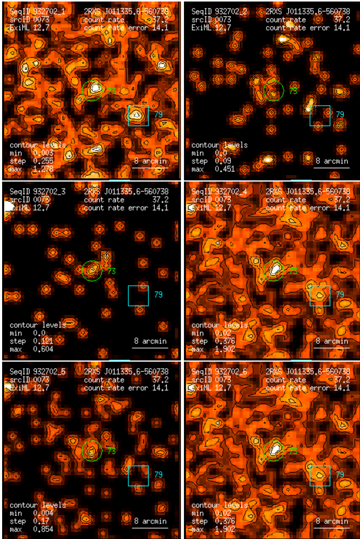
Figure 73: RASS 932702: detection 0073: band rate images, Gaussian filter: (1) PSPC channels 11 – 41, (2) 52 – 90, (3) 91 – 201, (4) 11 – 235, (5) 52 – 201, (6) 11 – 201. Broad band rates in counts/ks. Band rate contour levels in counts/ks/arcmin 2 .
