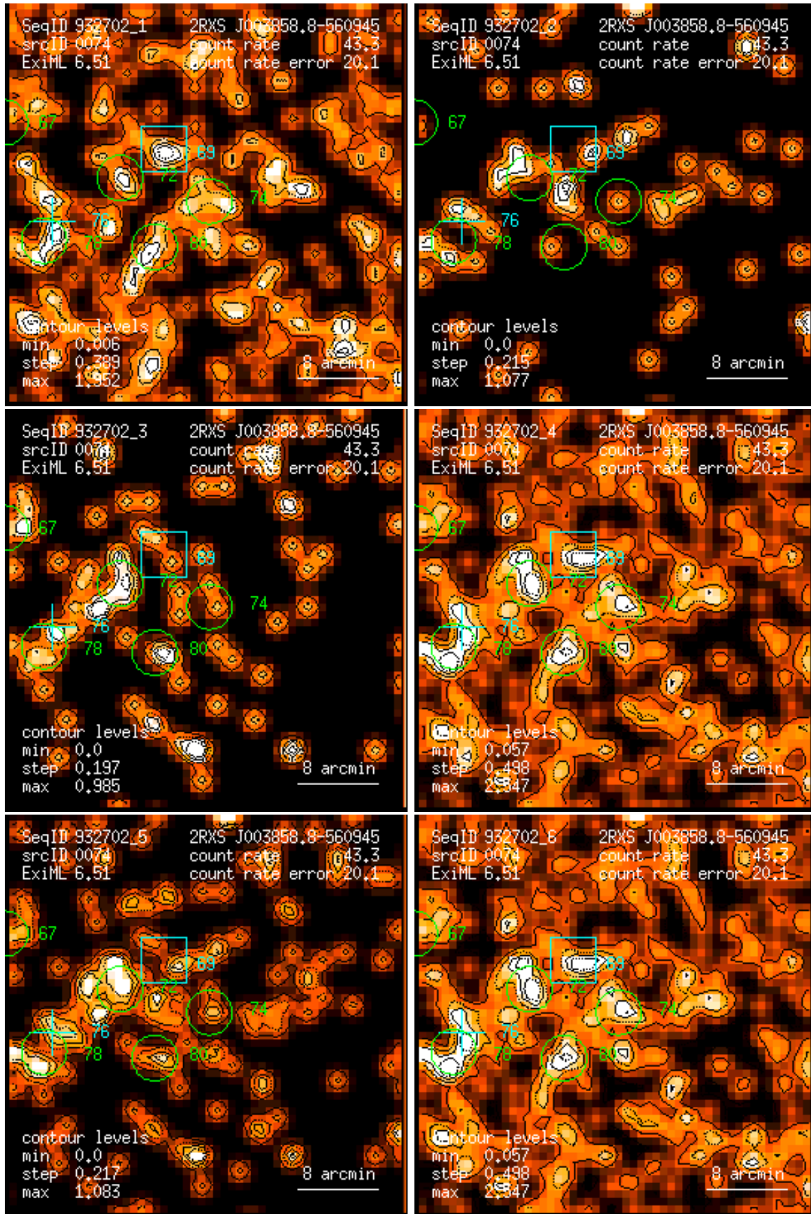
Figure 74: RASS 932702: detection 0074: band rate images, Gaussian filter: (1) PSPC channels 11 – 41, (2) 52 – 90, (3) 91 – 201, (4) 11 – 235, (5) 52 – 201, (6) 11 – 201. Broad band rates in counts/ks. Band rate contour levels in counts/ks/arcmin 2 .
