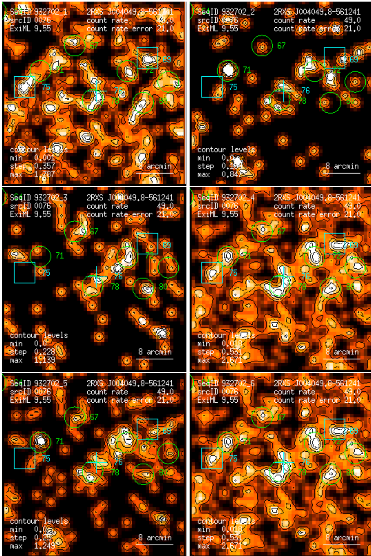
Figure 76: RASS 932702: detection 0076: band rate images, Gaussian filter: (1) PSPC channels 11 – 41, (2) 52 – 90, (3) 91 – 201, (4) 11 – 235, (5) 52 – 201, (6) 11 – 201. Broad band rates in counts/ks. Band rate contour levels in counts/ks/arcmin 2 .
